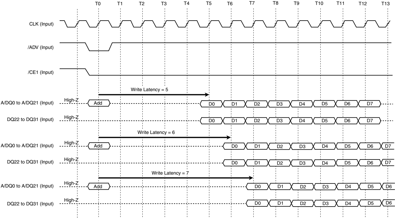
Figure 3-2. Latency Configuration (Write)
