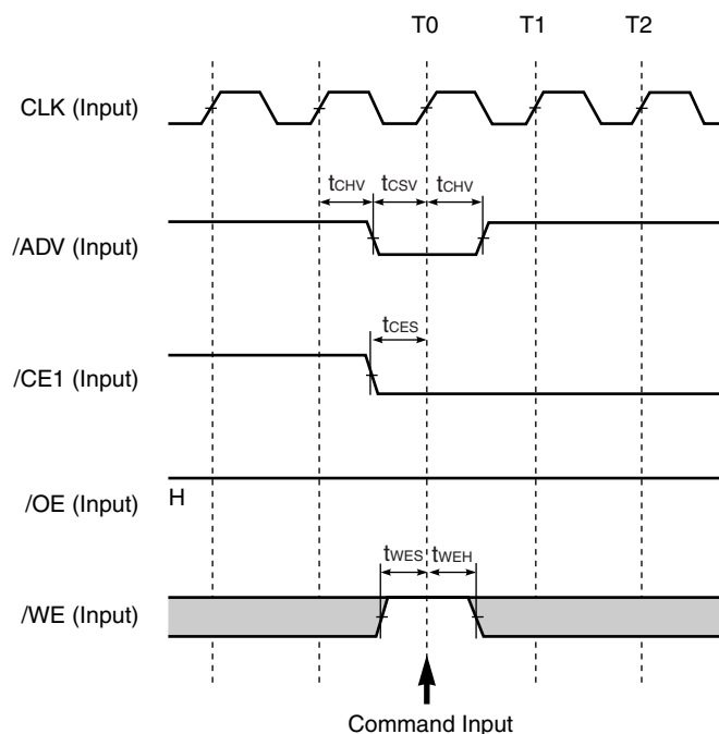
Figure 5-5. Command Loading Timing 1
