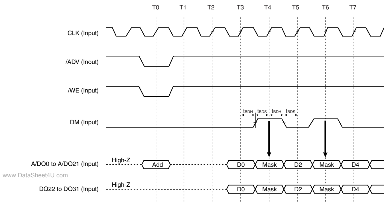
Figure 5-10. Command Loading Timing 1
