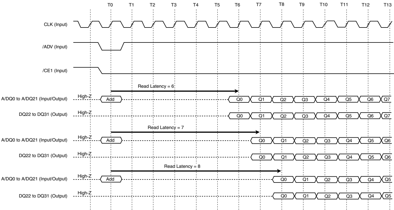
Figure 3-1. Latency Configuration (Read)
