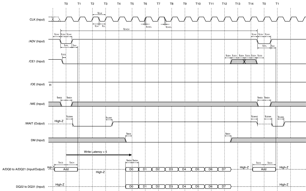
Figure 7-4. Burst Write Cycle Timing Chart (/CE1 Toggle Access)
