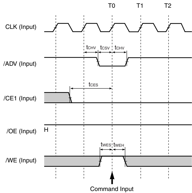
Figure 5-6. Command Loading Timing 2
