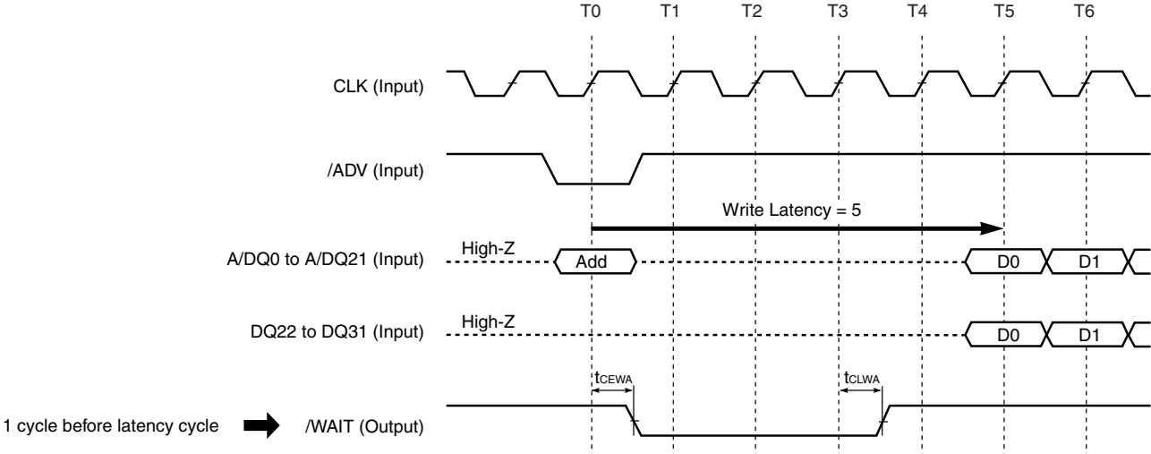
Figure 3-8. /WAIT Output Timing (Write Cycle)
