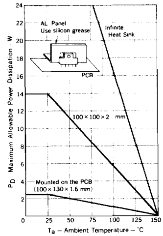
MAXIMUM ALLOWABLE POWER DISSIPATION vs. AMBIENT TEMPERATURE
