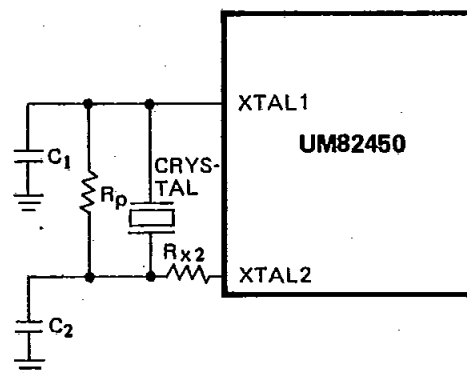
Typical Crystal Oscillator Network
