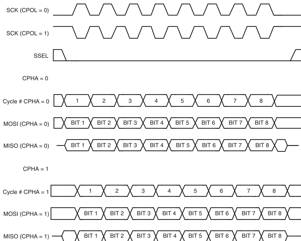
Fig 49. SPI data transfer format (CPHA = 0 and CPHA = 1)
