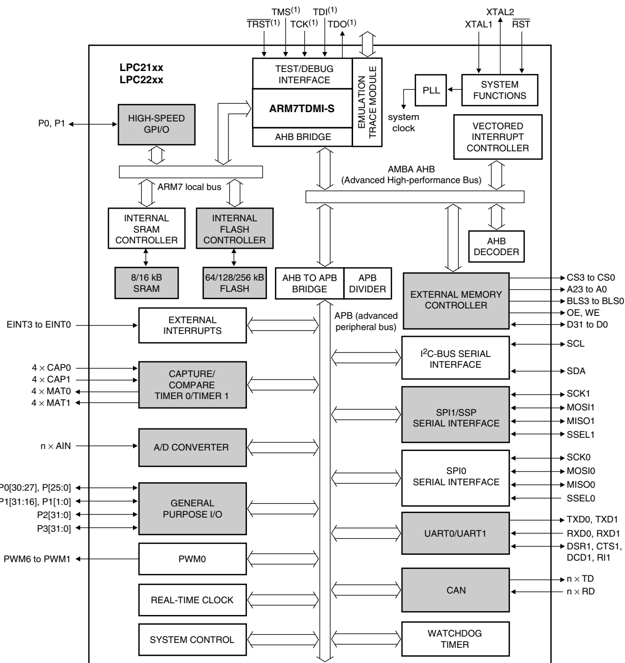
Fig 1. LPC21xx and LPC22xx block diagram
