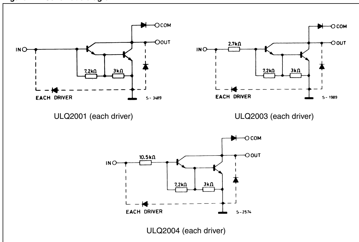
Figure 1. Schematic diagram
