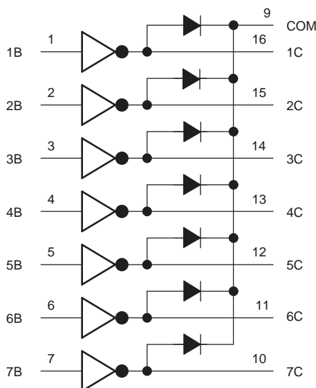
Simplified Schematic
