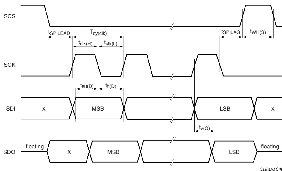
Fig 15. SPI timing diagram
