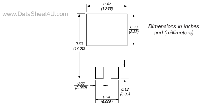
Mounting Pad Layout TO-263AB
