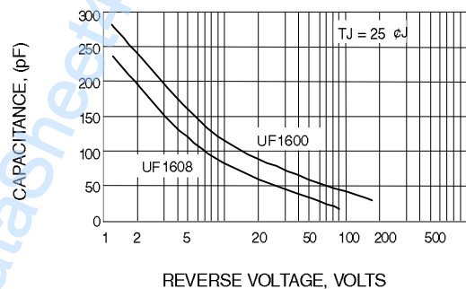
Fig. 4-TYPICAL JUNCTION CAPACITANCE
