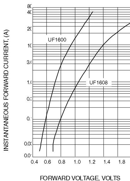
Fig. 5-TYPICAL FORWARD CHARACTERISTICS
