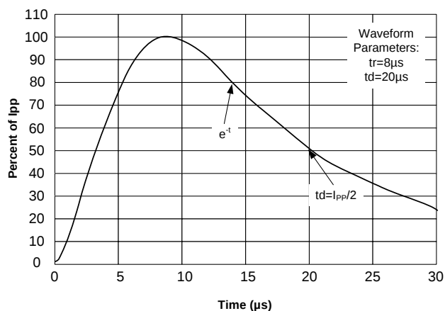
Pulse Waveform
