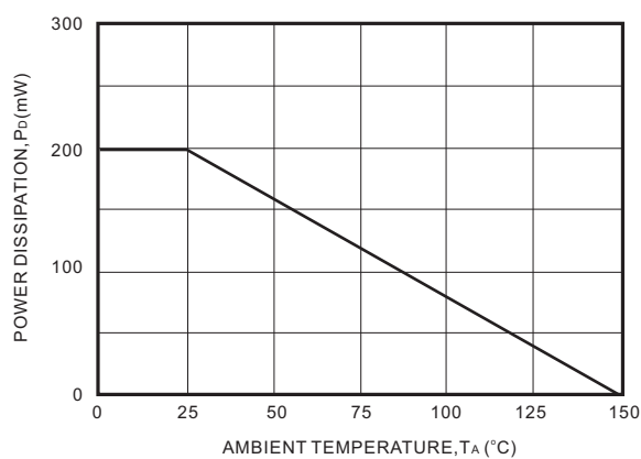
FIG. 2-DRATING CURVE
