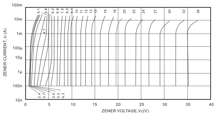
FIG.1-ZENER VOLTAGE CHARACTERISTICS
