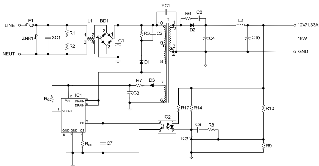
Fig.7 UTC UCS1600S Typical Application Circuit
