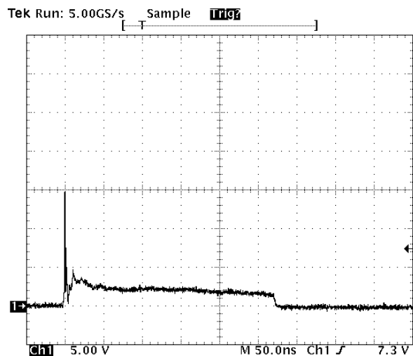
ESD Clamping (15kV air per IEC 61000-4-2)
