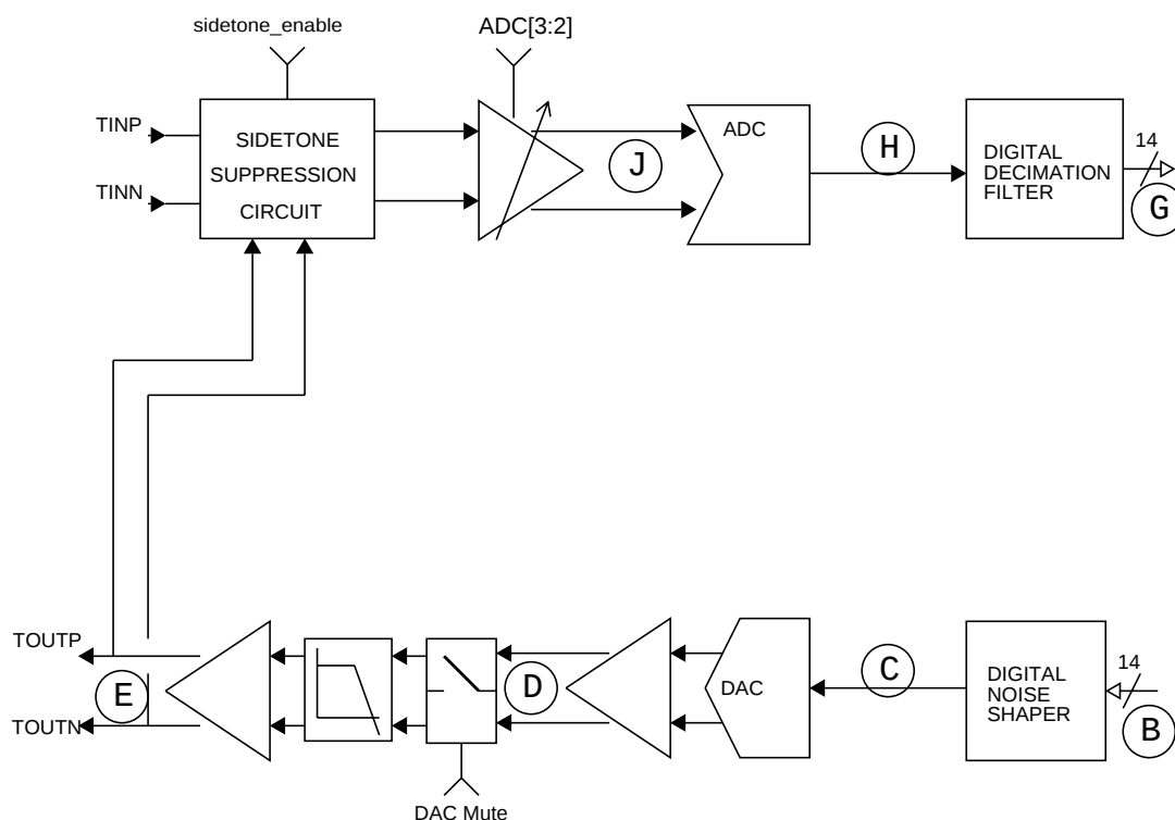
Fig 3. Telecom codec block diagram
