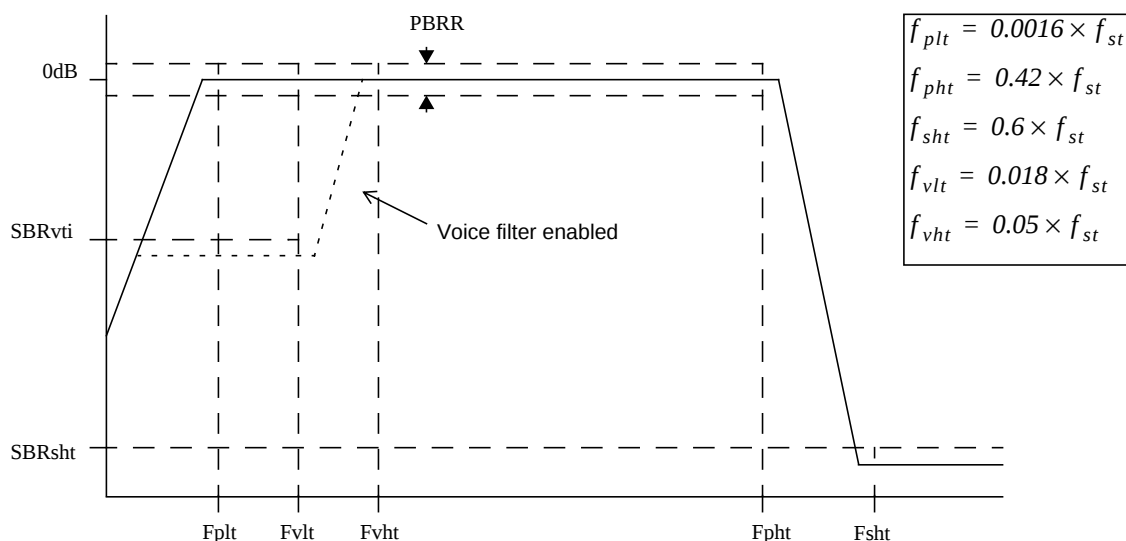
Fig 10. Telecom input frequency response
