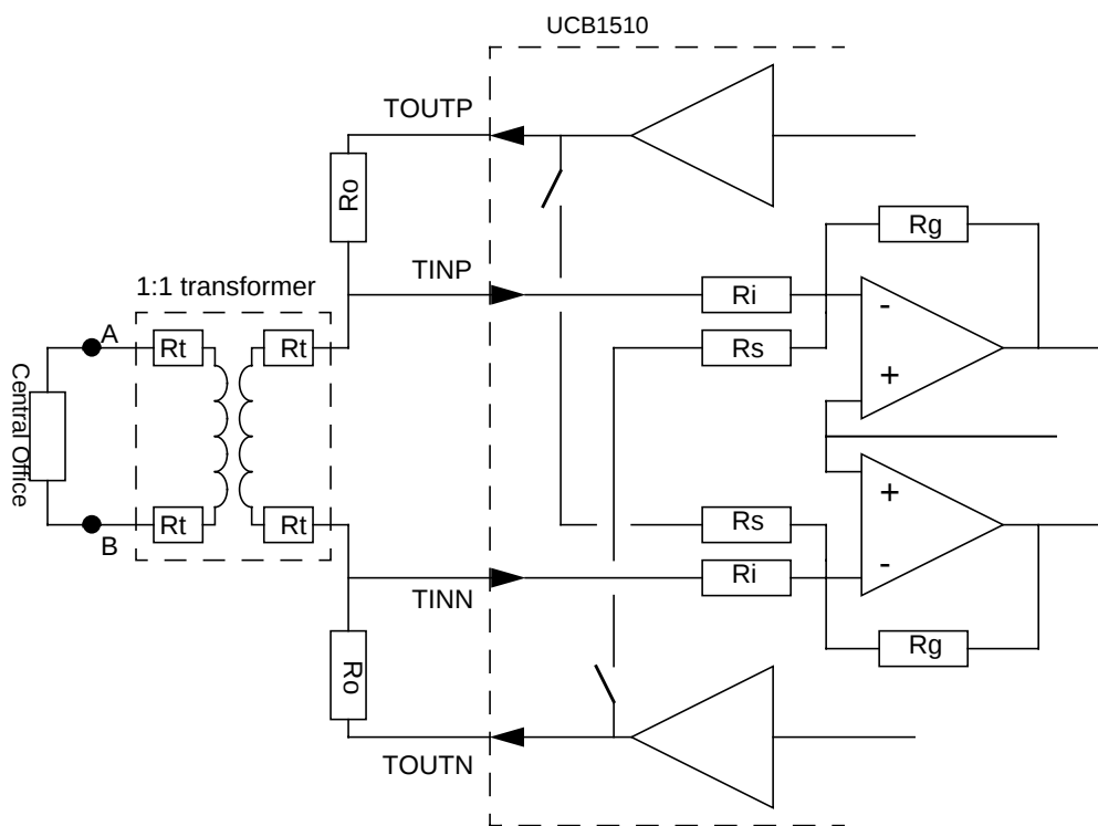
Fig 4. Typical telecom codec sidetone suppression circuit (without protection circuits).
