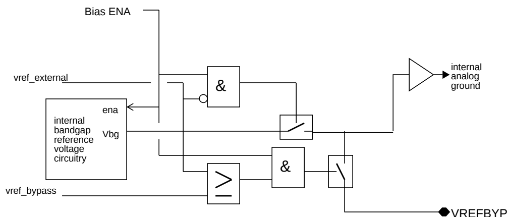
Fig 5. Block diagram of the reference circuit.
