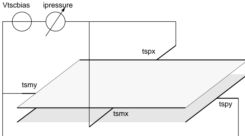
Fig.9 Touch screen setup for pressure measurement.
