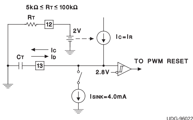
Figure 1. Oscillator
