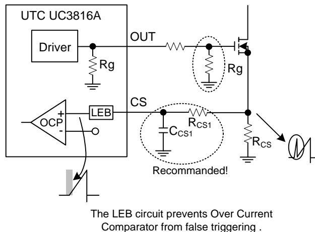
Fig. 7 Current Sensing
