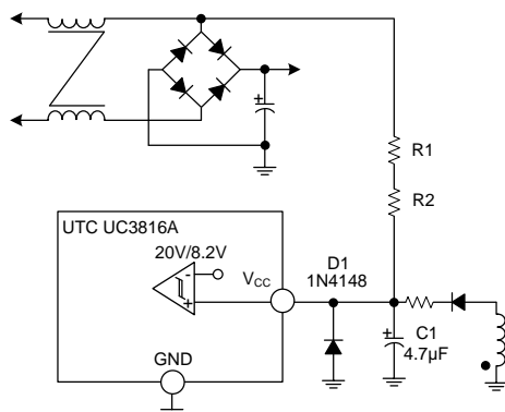
Fig. 1 Startup Circuit
