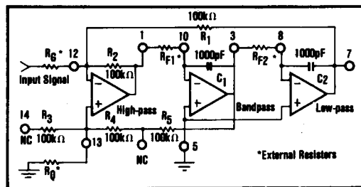
FIGURE 3. Inverting Configuration.
