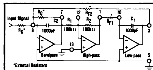
FIGURE 4. Bi-Quad Configuration.
