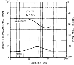
FORWARD TRANSADMITTANCE AS A FUNCTION OF FREQUENCY
