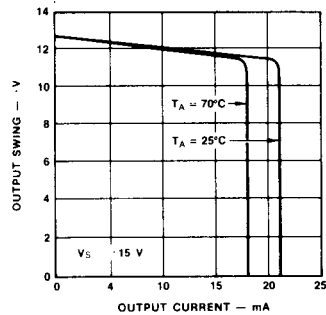
Current Limiting
