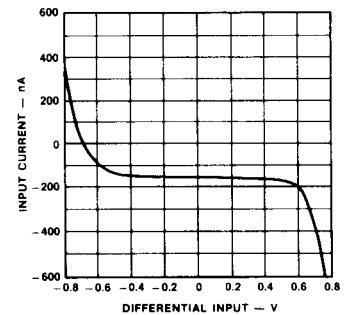
Input Current
