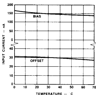
Input Current
