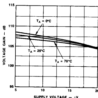
Voltage Gain
