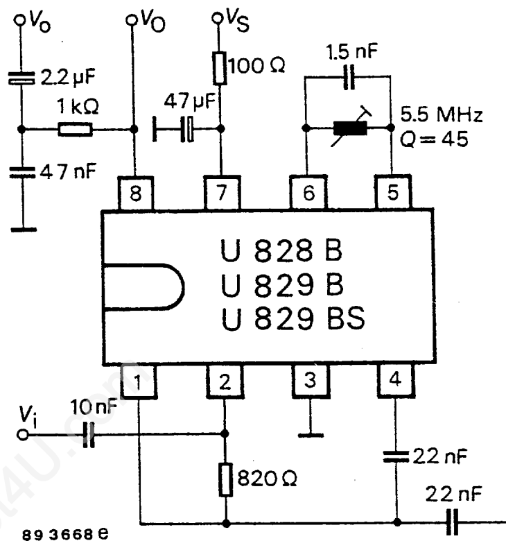
Figure 4. Test circuit
