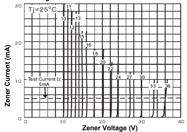
Fig.6- Zener Breakdown Characteristics
