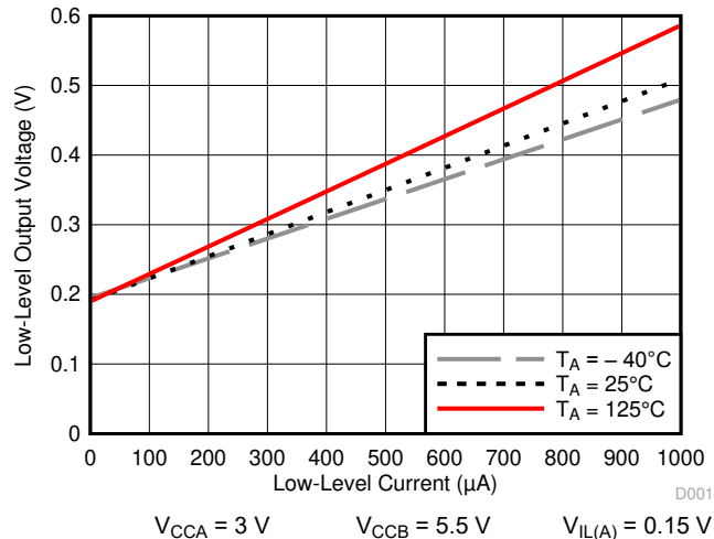
Figure 7-2. Low-Level Output Voltage ( V_{OL(Bx)} ) vs Low-Level Current ( I_{OL(Bx)} )
