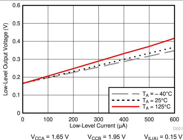
Figure 7-3. Low-Level Output Voltage ( V_{OL(Bx)} ) vs Low-Level Current ( I_{OL(Bx)} )
