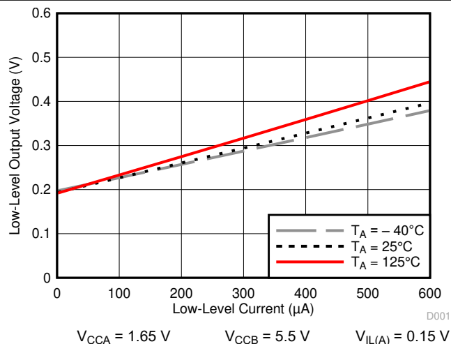
Figure 7-4. Low-Level Output Voltage ( V_{OL(Bx)} ) vs Low-Level Current ( I_{OL(Bx)} )
