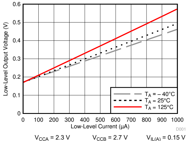
Figure 7-1. Low-Level Output Voltage ( V_{OL(Bx)} ) vs Low-Level Current ( I_{OL(Bx)} )
