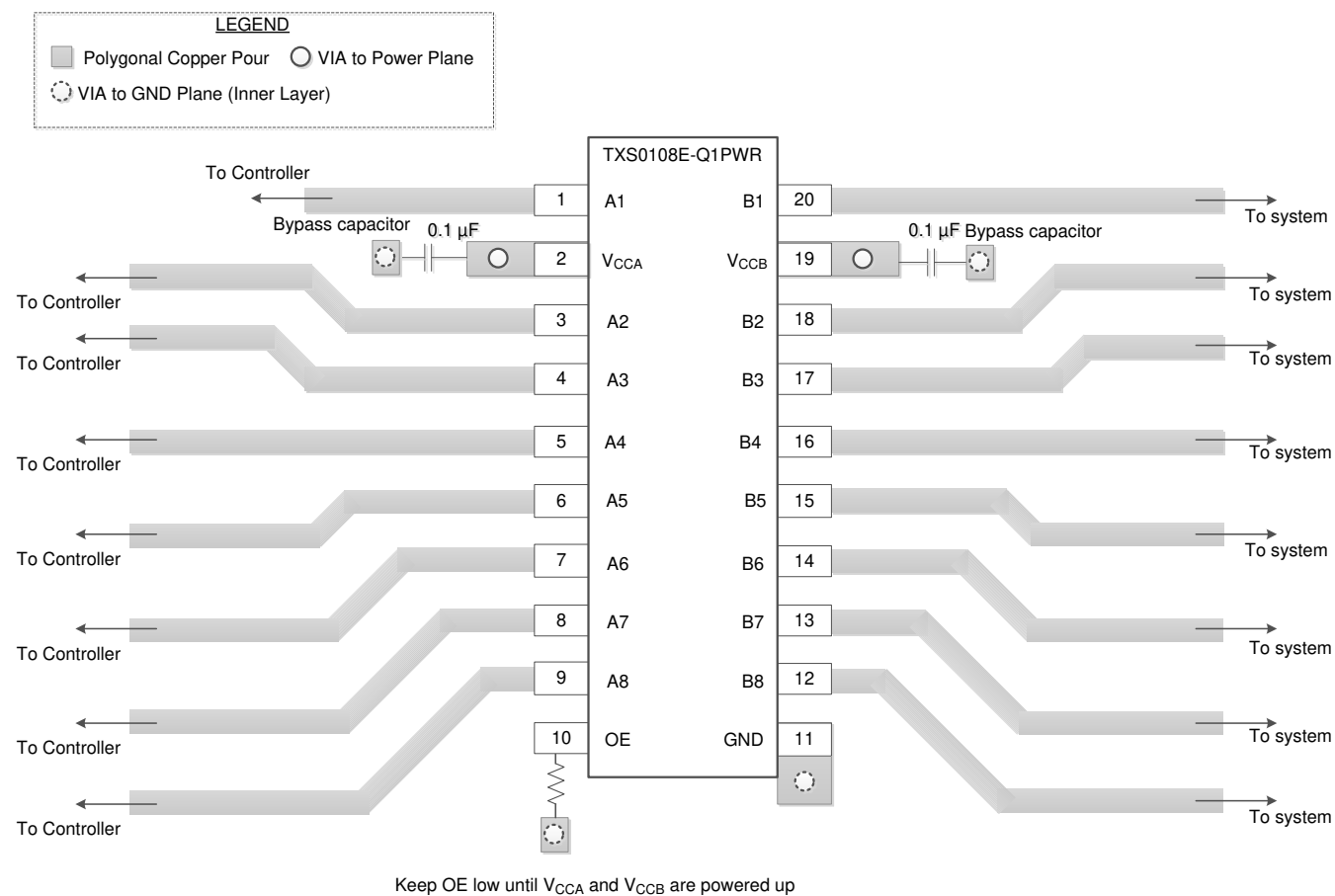
Figure 10-3. Layout Example
