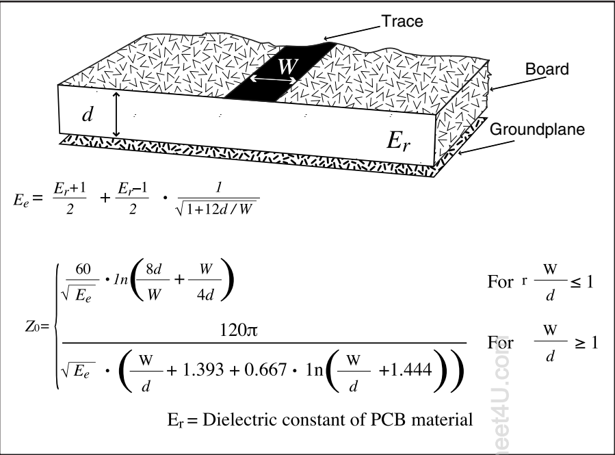
Figure 13: Microstrip Formulas ( E_r = dielectric constant of PC board material)
