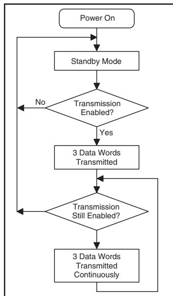
Figure 8: Encoder Flowchart
