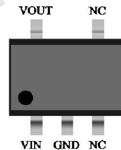
SOT23-5(Top view)
