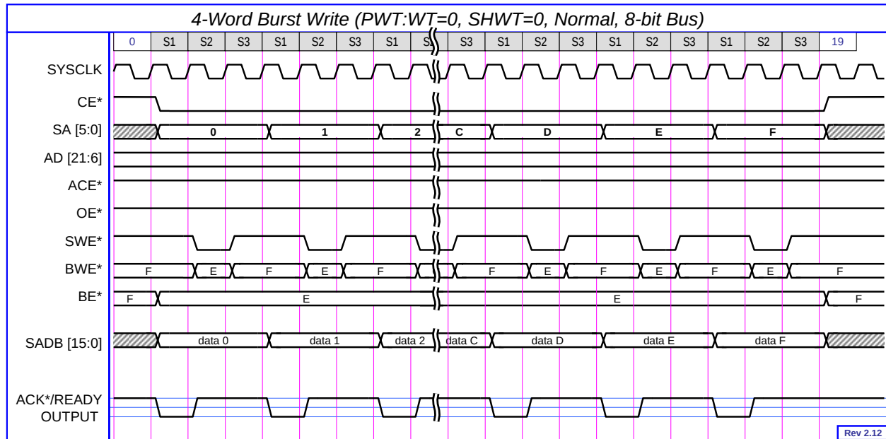
Figure 9-26 4-word Burst Write (PWT: WT=0, SHWT=0, Normal, 8-bit Bus)
