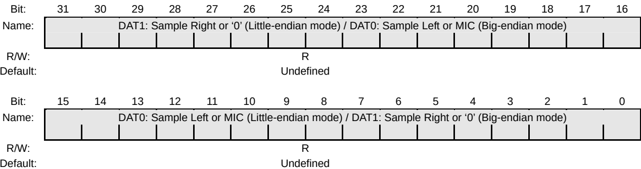
Figure 24-23 ACAUDIDAT Register
