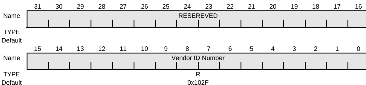
Figure 18-19 Vendor ID Register
