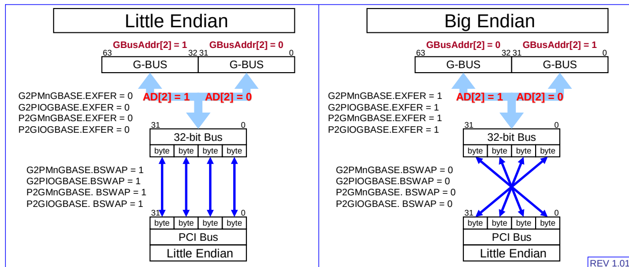
Figure 16-10 Endian Switching.
