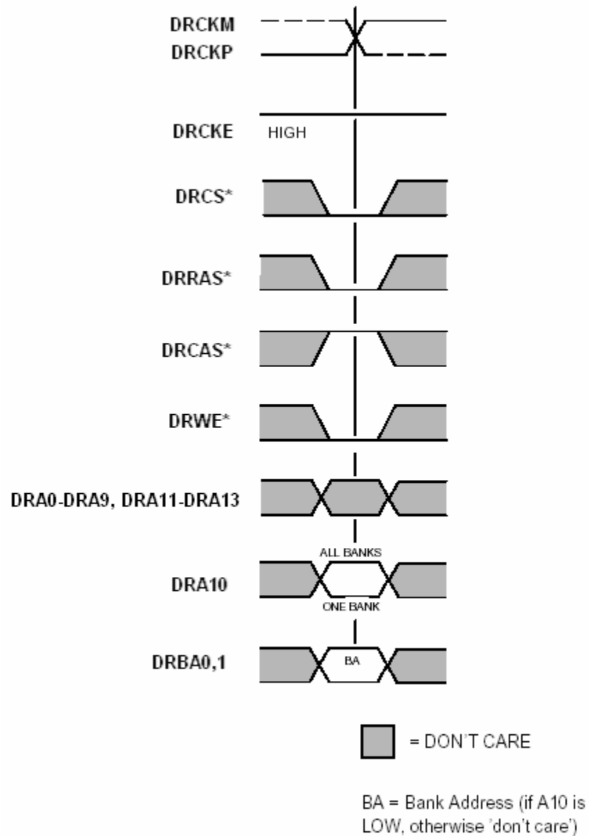
Figure 15-5 Precharge Command
