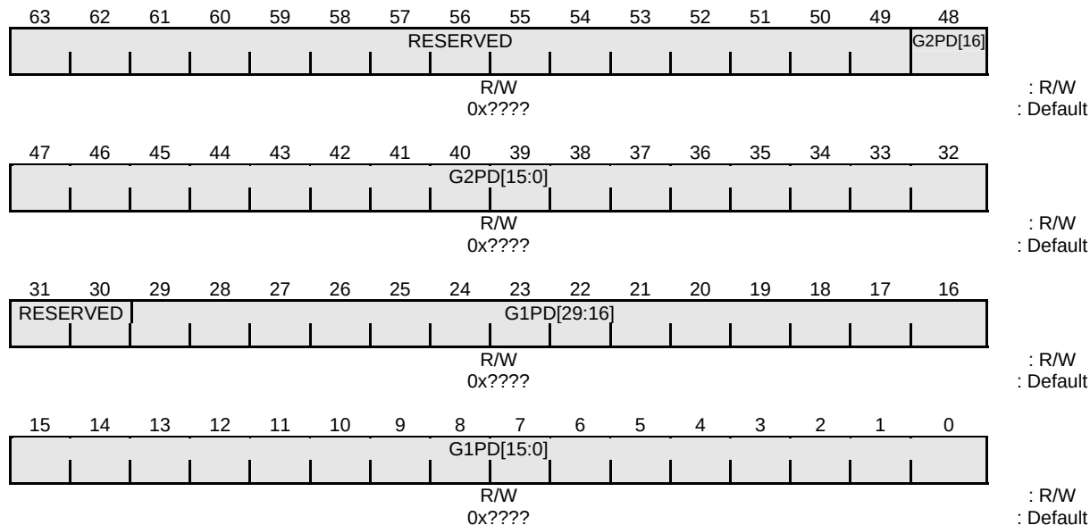
Figure 7-14 GPIODR2 Register
