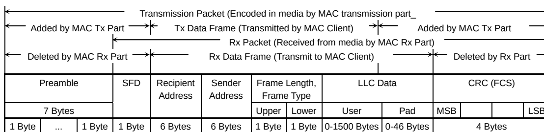
Figure 18-10 Ethernet Packet Frame Fields
