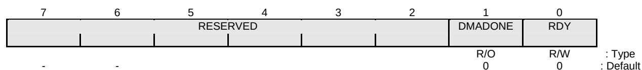
Figure 10-12 NAND Flash Memory Interrupt Status Register (NDFISR)
