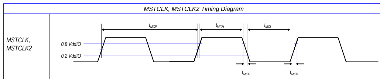
Figure 28-1 MSTCLK Timing Diagram
