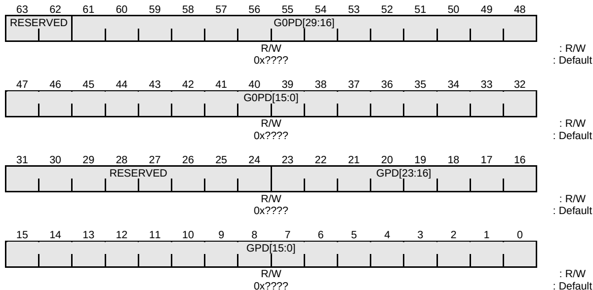
Figure 7-12 GPIODR1 Register
