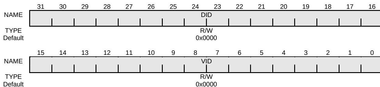
Figure 16-64 ID Register
