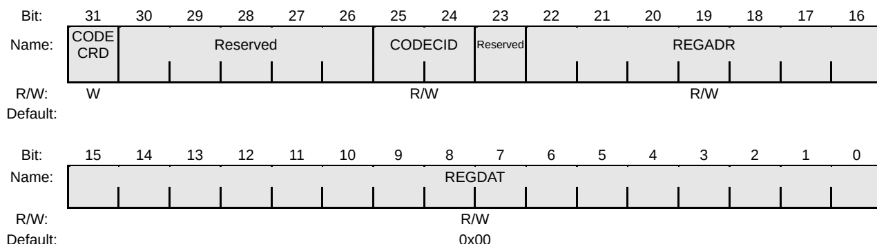
Figure 24-11 ACREGACC
