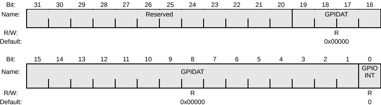
Figure 24-14 ACGPIDAT Register
