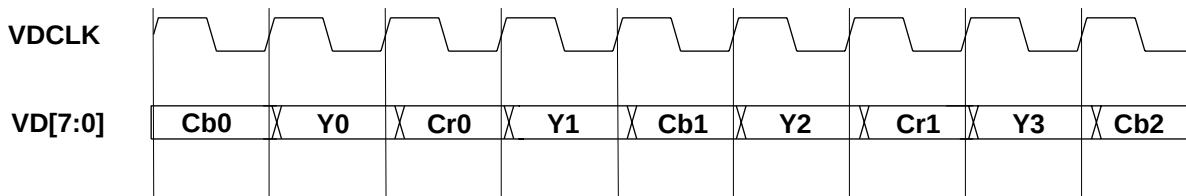
Figure 12-2 ITU.BT656 (CCIR656) Digital Video Timing
