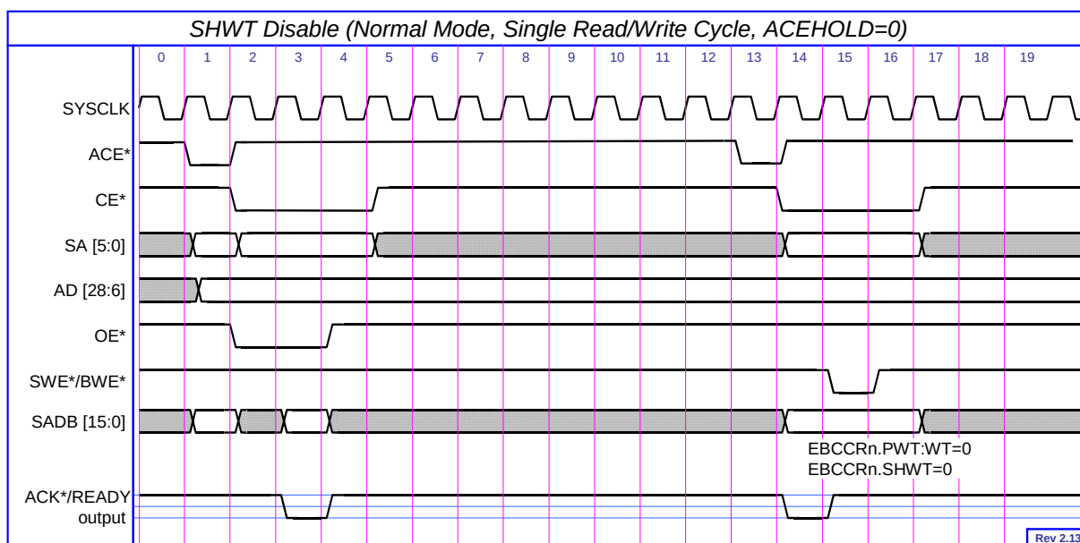
Figure 9-6 SHWT Disable (Normal Mode, Single Read/Write Cycle)
