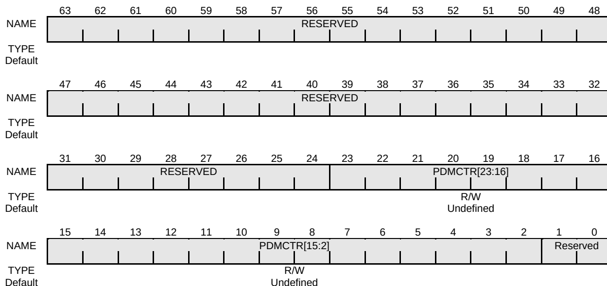
Figure 16-71 Count Register
