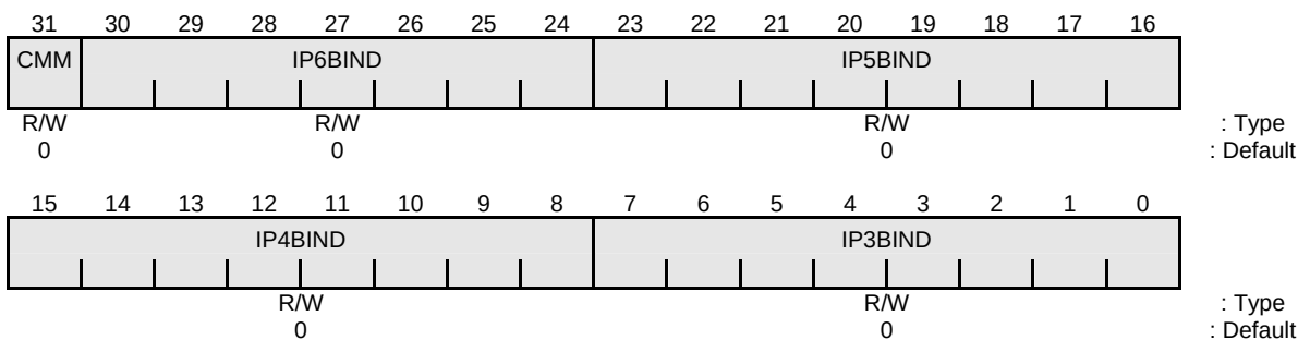
Figure 8-5 Interrupt Source and Cause IP Binding Register
