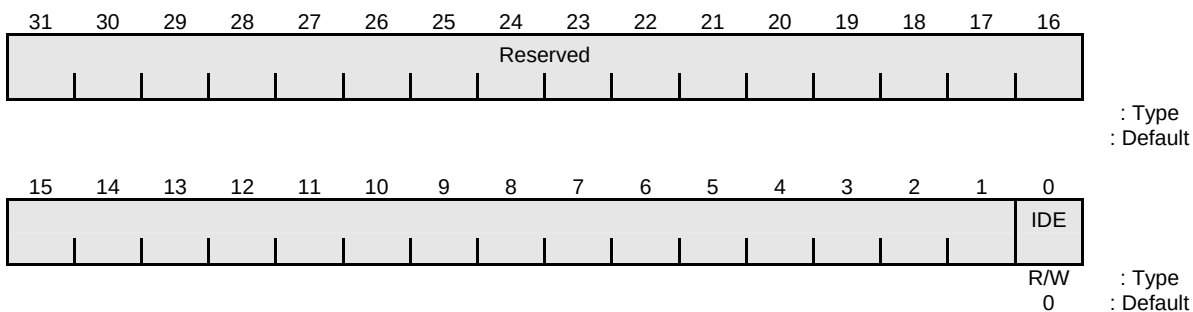
Figure 8-4 Interrupt Detection Enable Register
