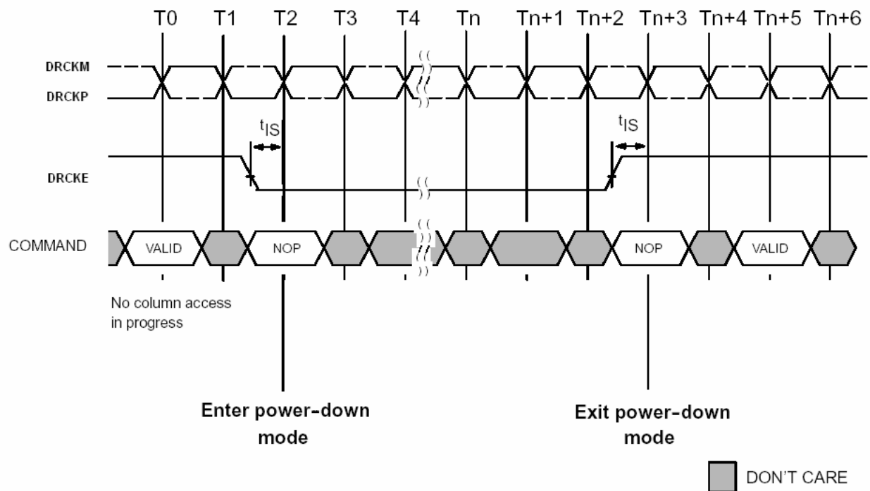
Figure 15-6 Power-Down Command
