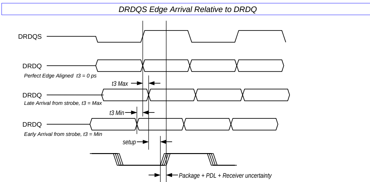
Figure 28-9 DRDQS Edge Arrival Relative to DRDQ
