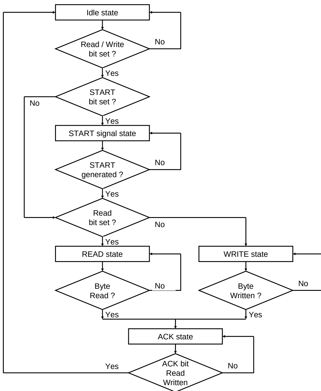
Figure 22-5 Control Flow
