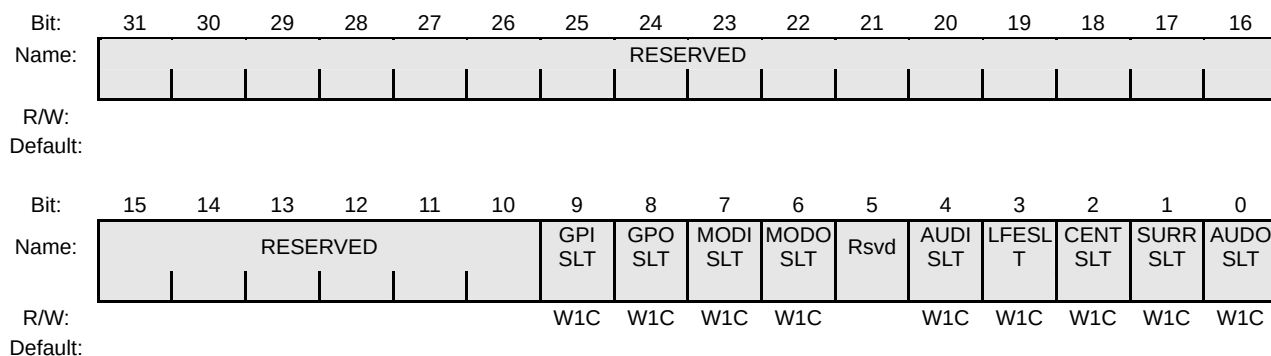
Figure 24-17 ACSLTDIS Register
