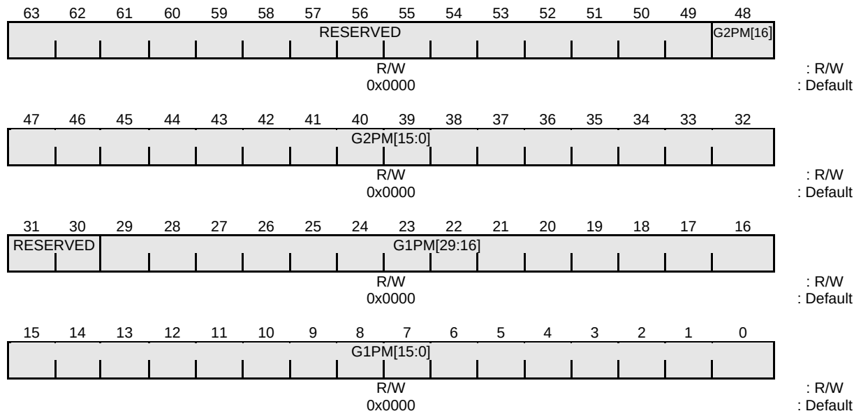
Figure 7-13 GPIOMR2 Register
