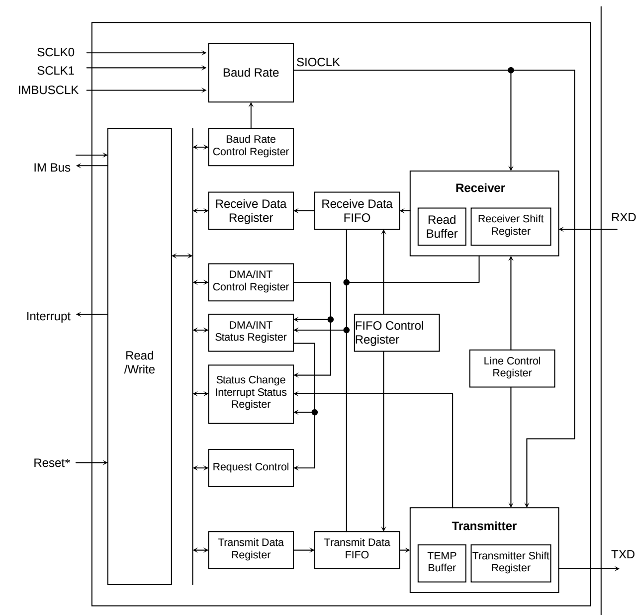
Figure 19-1 SIO Internal Block Diagram
