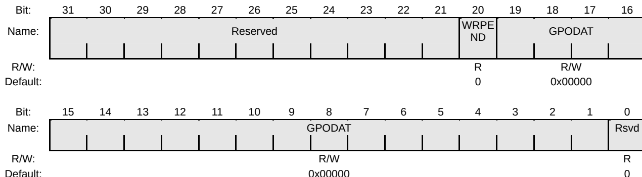
Figure 24-15 ACGPODAT Register
