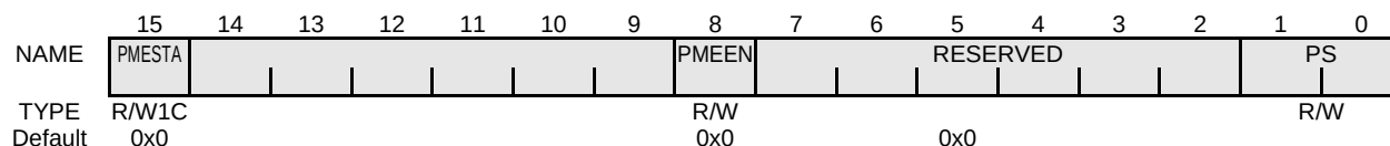
Figure 16-80 PMCSR Register
