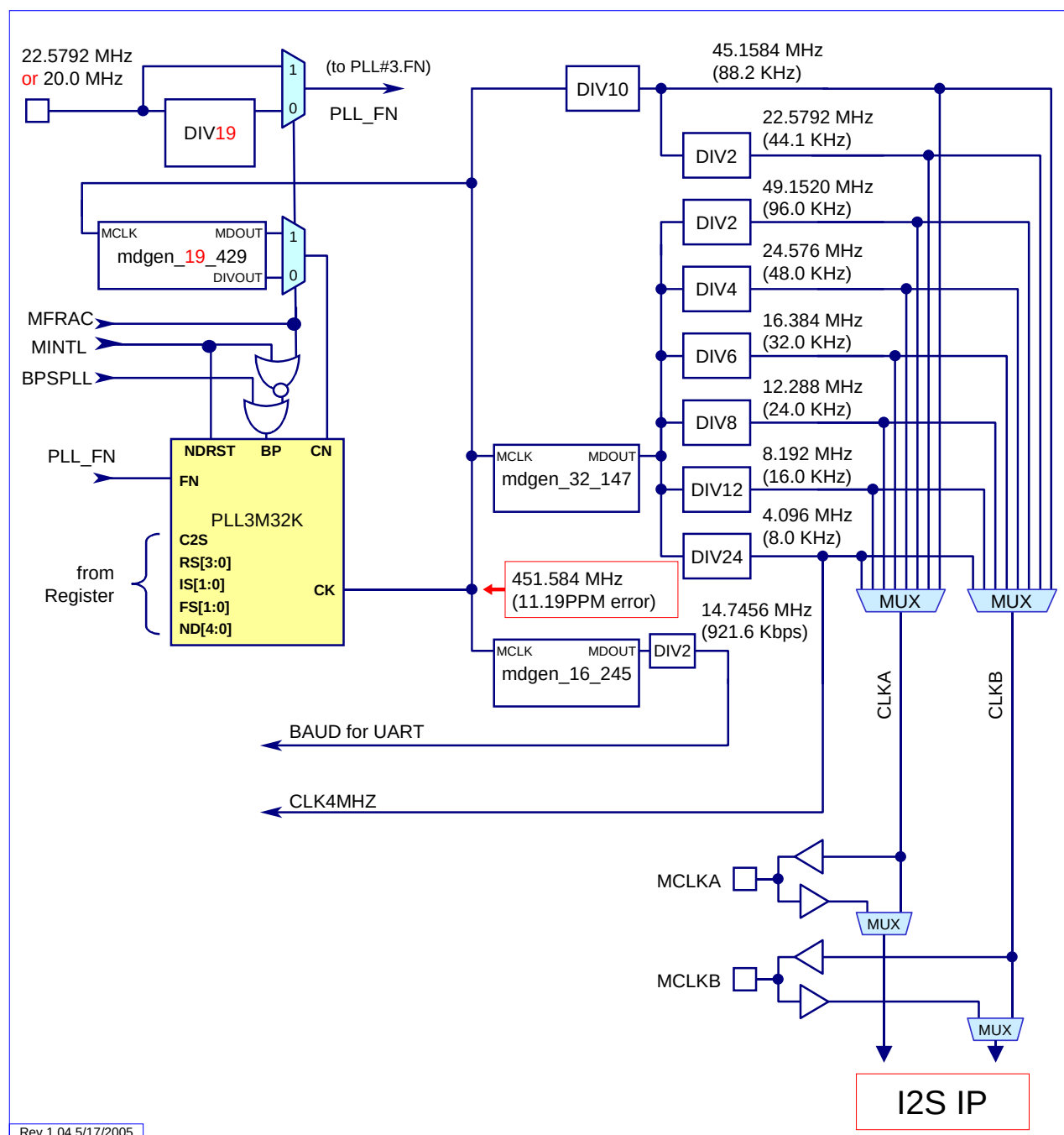
Figure 5-3 Diagram of Audio Clock Generator
