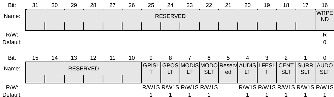
Figure 24-16 ACSLTEN Register
