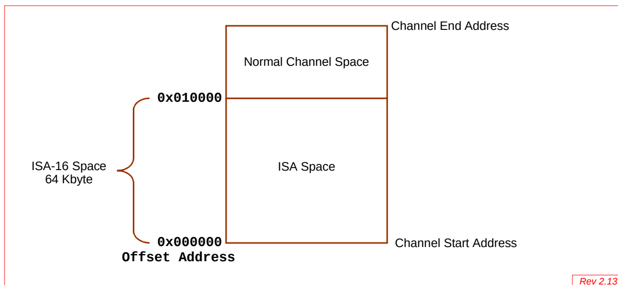
Figure 9-14 Physical Address Mapping of the ISA Spaces
