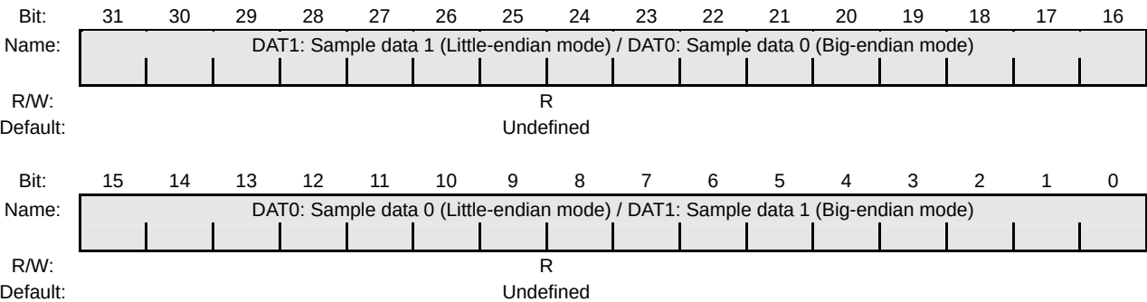
Figure 24-24 ACMODIDAT Register
