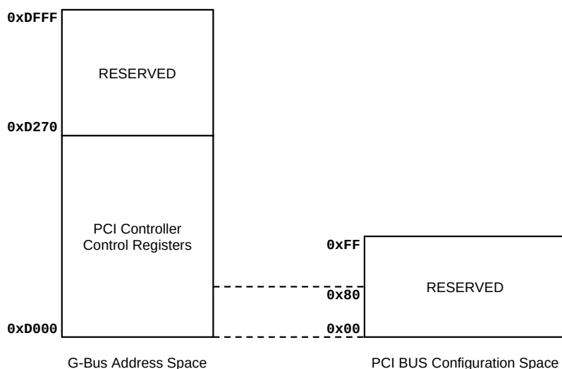
Figure 16-4 Register Map (Host Mode)
