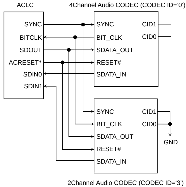
Figure 24-3 5.1 Channel Audio Connection Diagram
