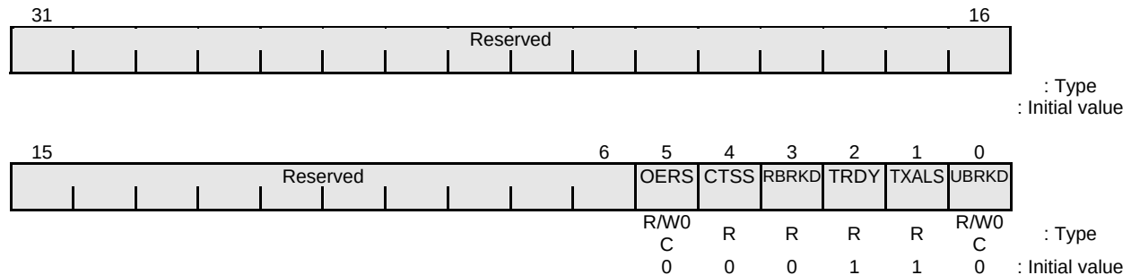
Figure 19-9 Status Change Interrupt Status Register
