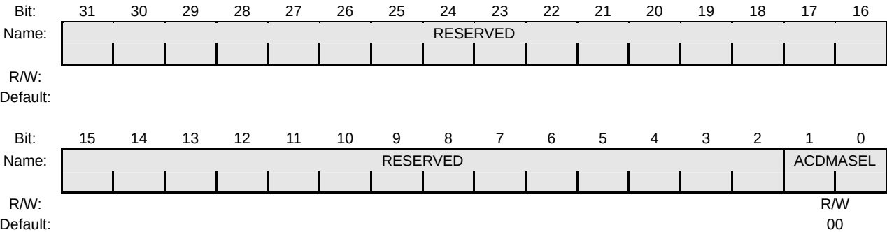
Figure 24-20 ACDMASEL Register
