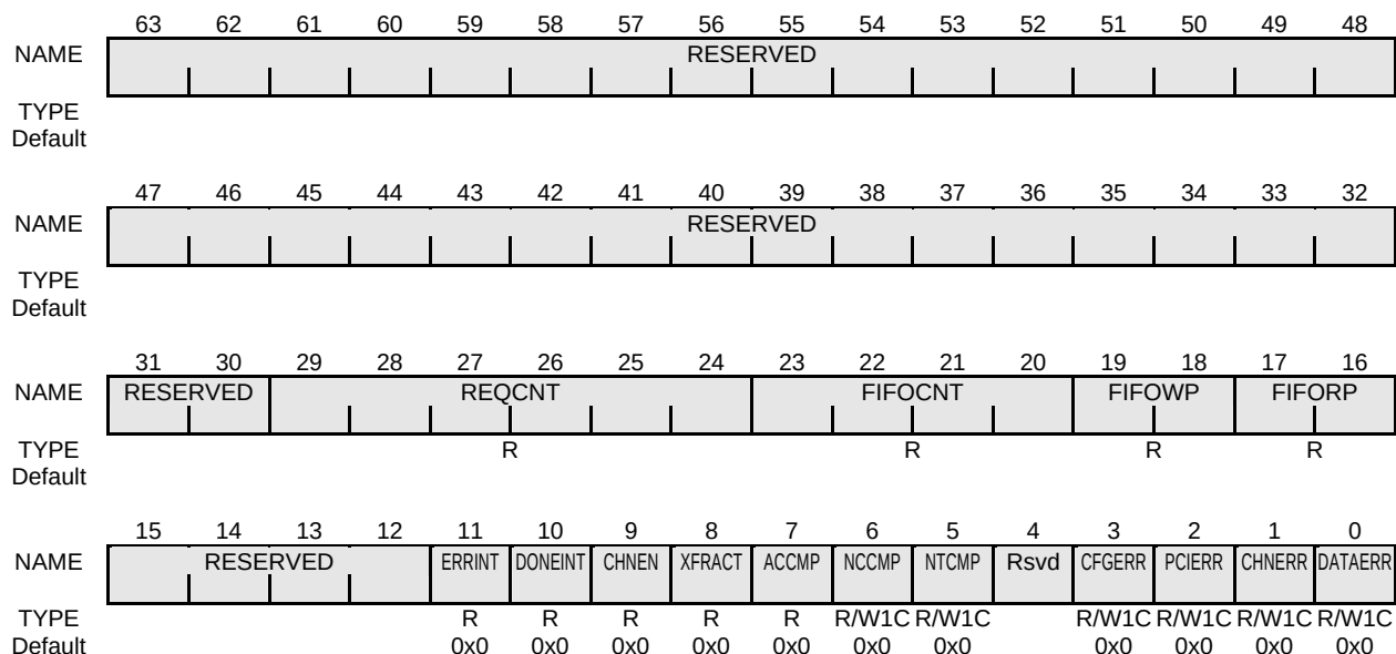
Figure 16-73 Status Register
