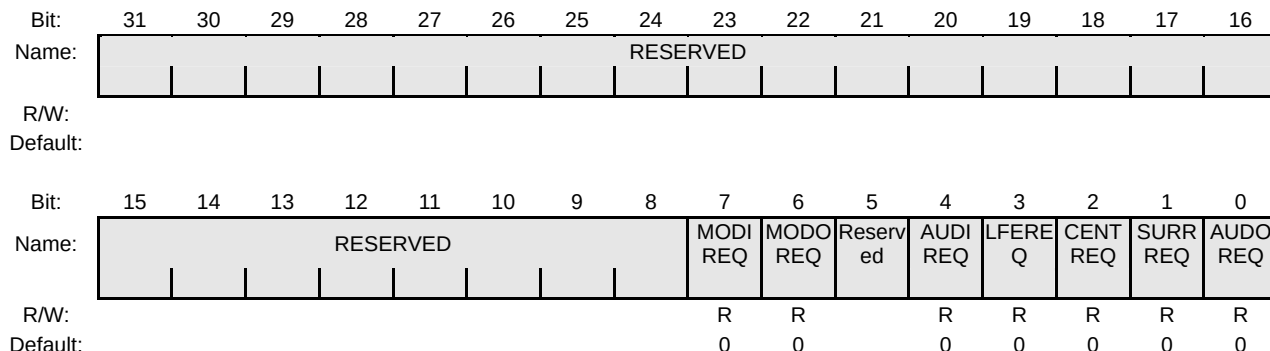
Figure 24-19 ACDMASTS Register
