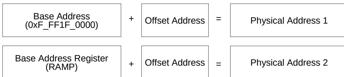
Figure 6-7 Generating Physical Address for a Internal Register
