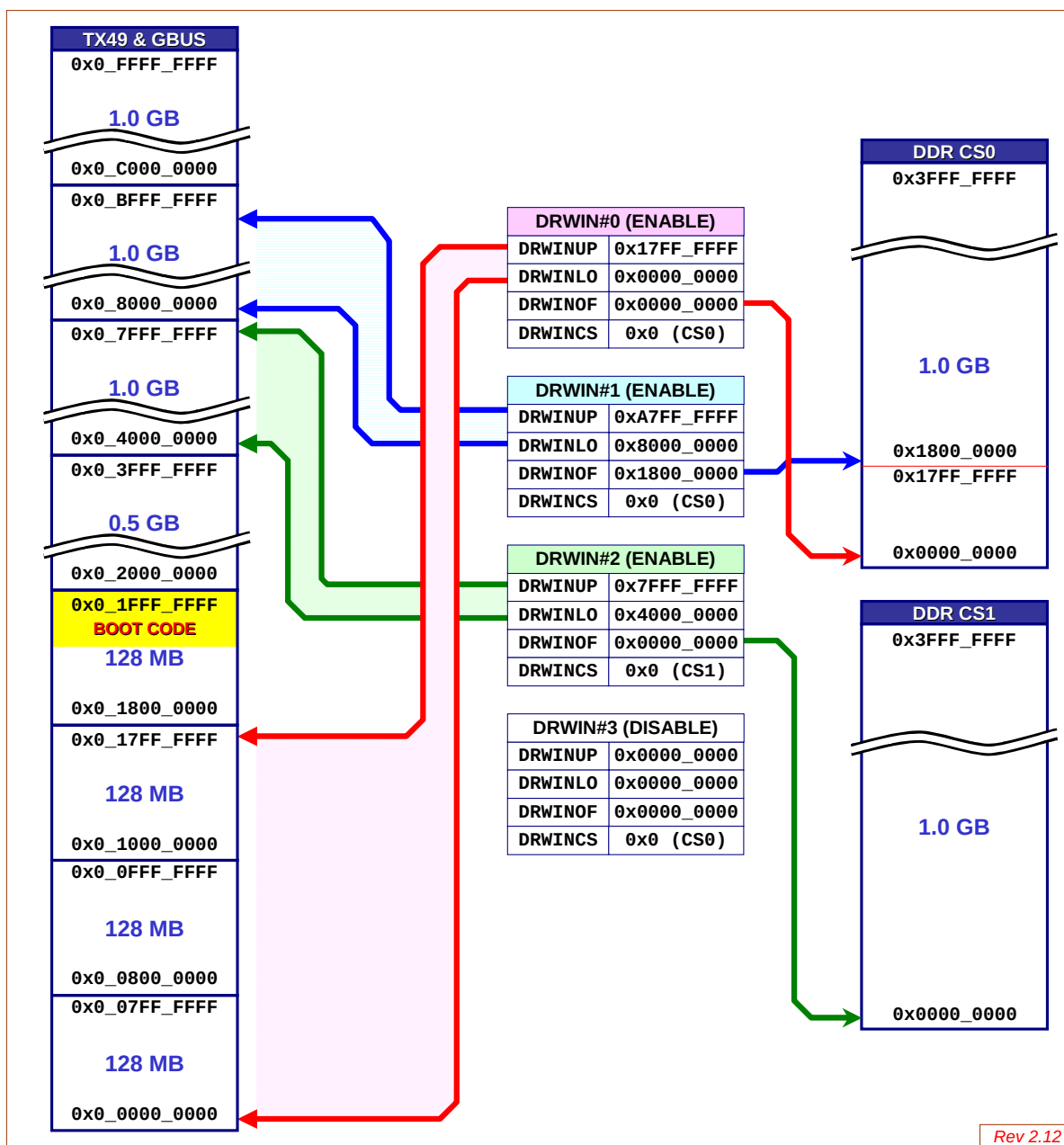
Figure 6-5 Example of DDR Memory Split-Mapping
