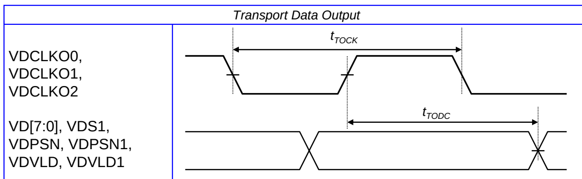
Figure 28-22 Video port Transport data output
