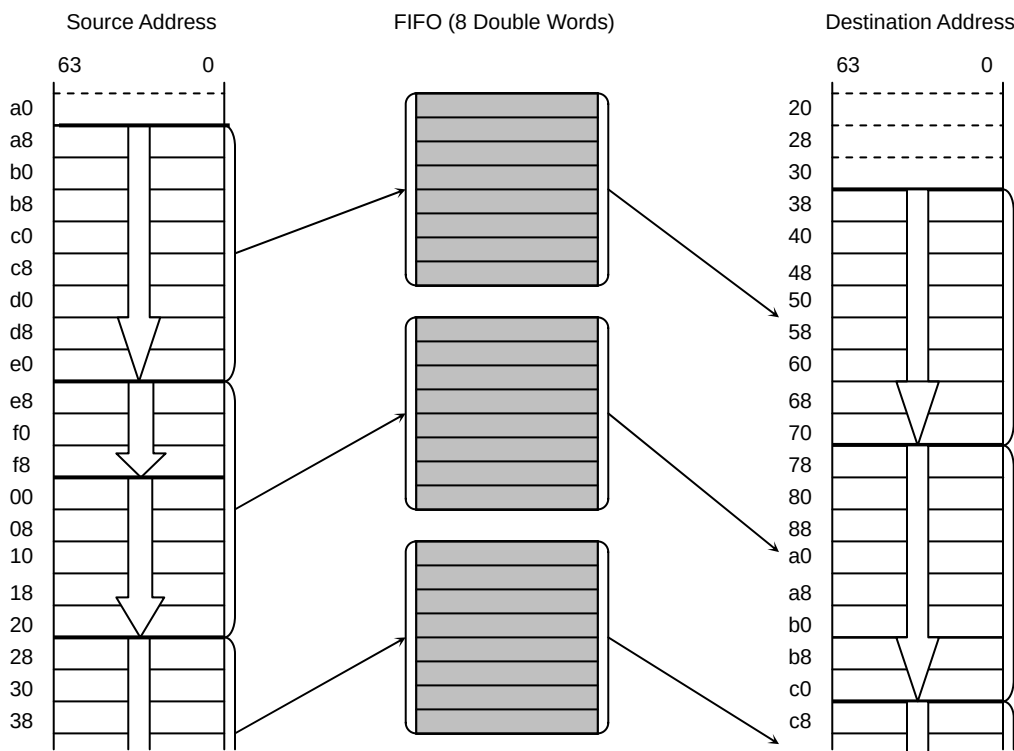
Figure 14-4 Dual Address Burst Transfer (DMCCRN.USEXFSZ = 1)
