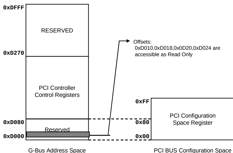
Figure 16-5 Register Map (Satellite Mode)
