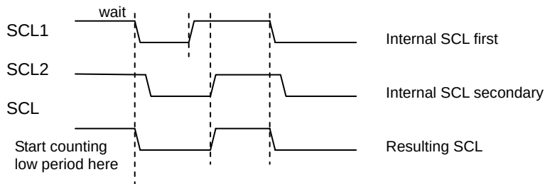
Figure 22-3 Clock Synchronization
