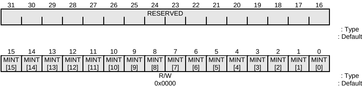
Figure 8-20 Interrupt Request Internal Interrupt Mask Register
