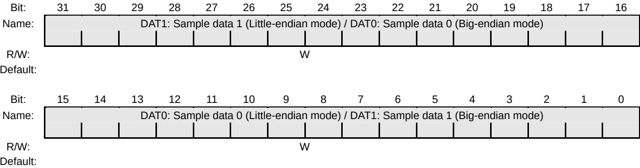
Figure 24-22 ACCENDAT/ACLFEDAT/ACMODODAT Register
