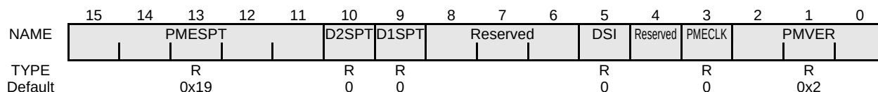
Figure 16-79 PMC Register
