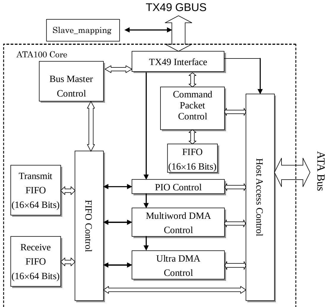
Figure 17-1 ATA100 Controller Block Diagram
