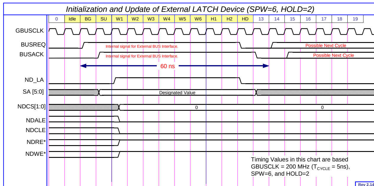
Figure 10-15 Initialization and Update Sequence
