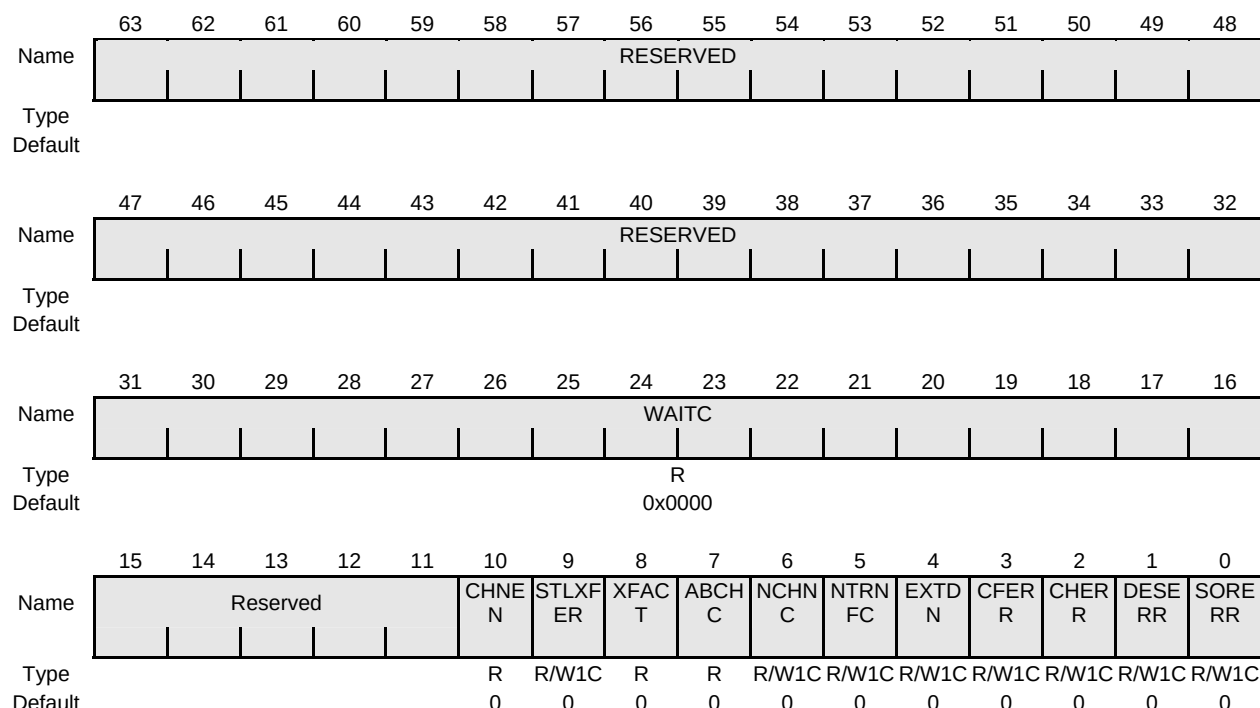
Figure 14-11 DMA Channel Status Register
