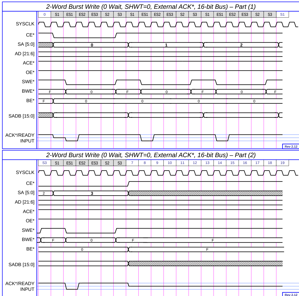
Figure 9-32 2-word Burst Write (0 Wait, SHWT=0, External ACK*, 16-bit Bus) (For 1/3 clock speed – SP=01, SADB setup time to assertion of SWE is ½ SYSCLK)
