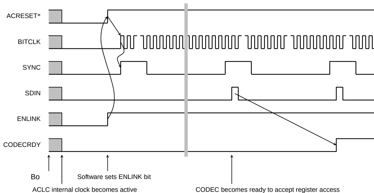
Figure 24-6 Cold Reset and CODEC Ready Recognition
