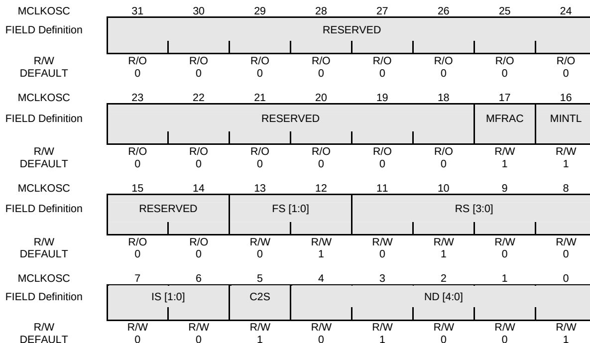
Figure 5-5 Definition of MCLKOSC Register
