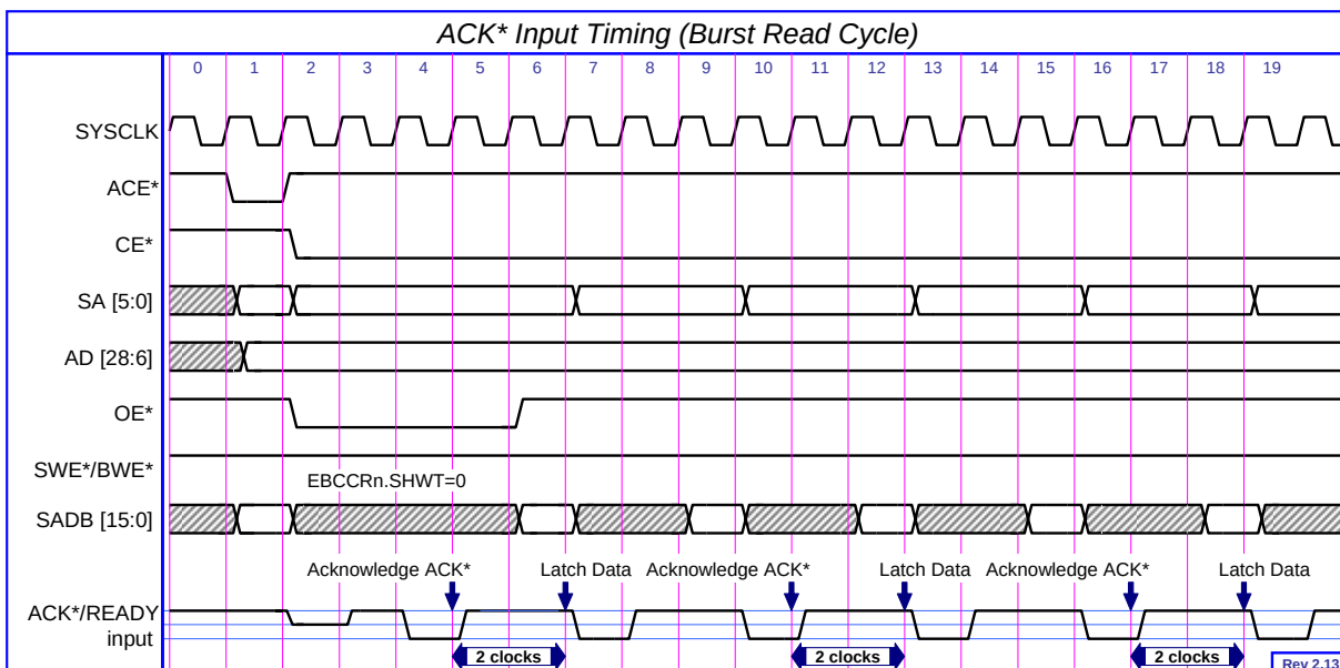
Figure 9-10 ACK* Input Timing (Burst Reade Cycle)
