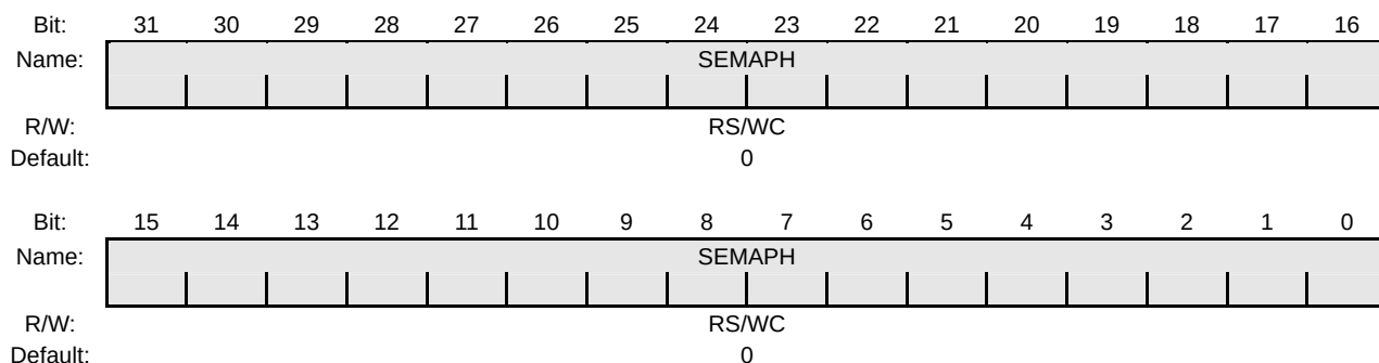
Figure 24-13 ACSEMAPH Register
