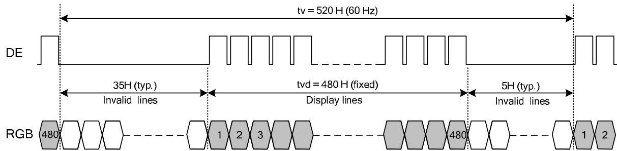
Fig. 9.2 Vertical Timing
