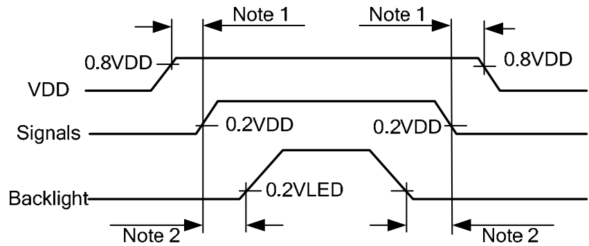
Fig. 9.4 Power Sequence Timing
