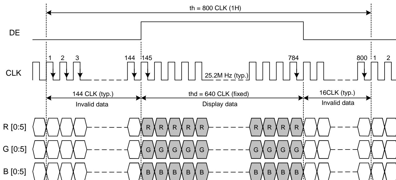
Fig. 9.3 Horizontal Timing of DE Mode
