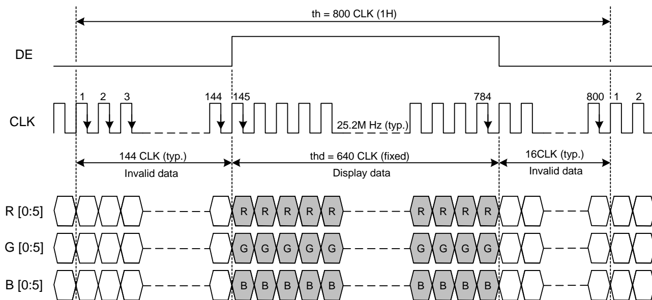
Fig. 9.3 Horizontal Timing of DE Mode
