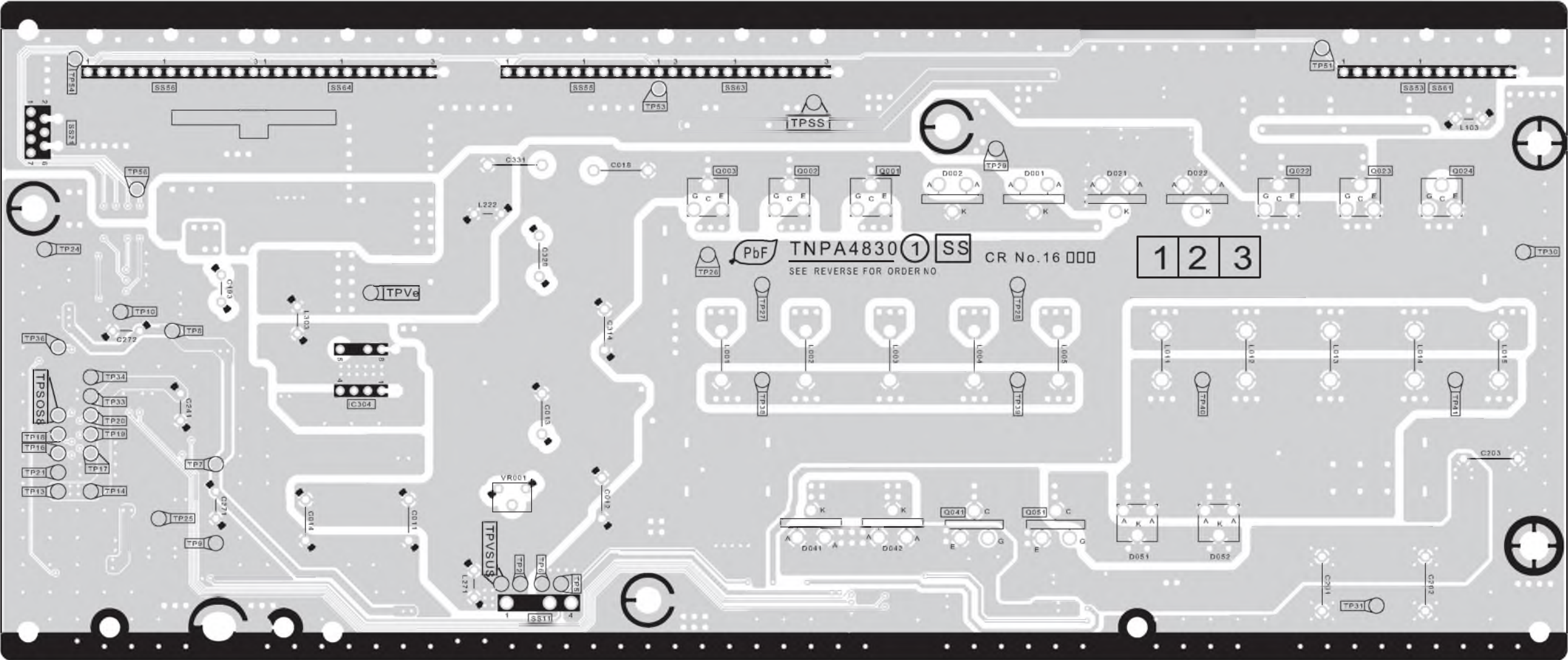
SS-BOARD (FOIL SIDE) TXNSS11XBH
