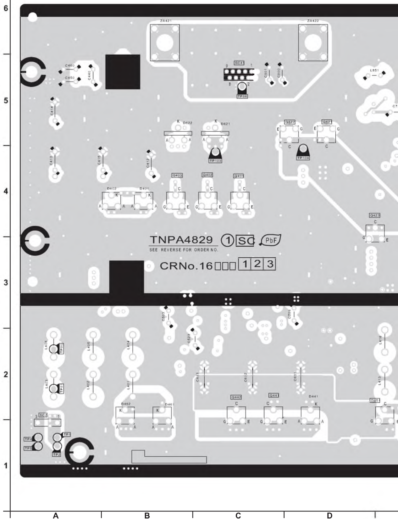
SC-BOARD (FOIL SIDE) TXNSC11XBH
