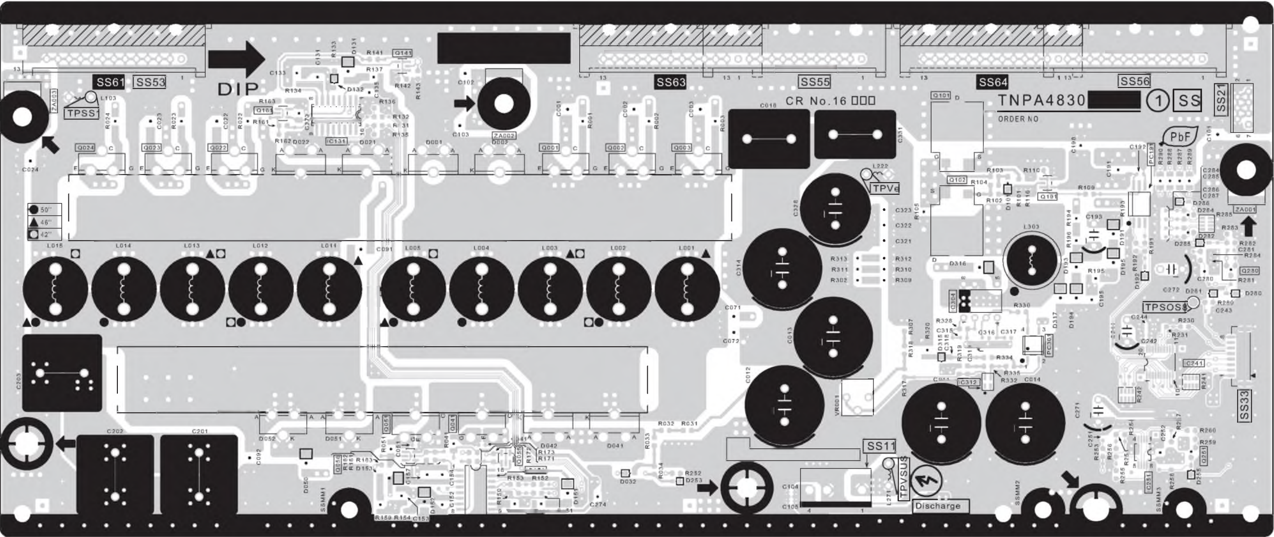
SS-BOARD (COMPONENT SIDE) TXNSS11XBH
