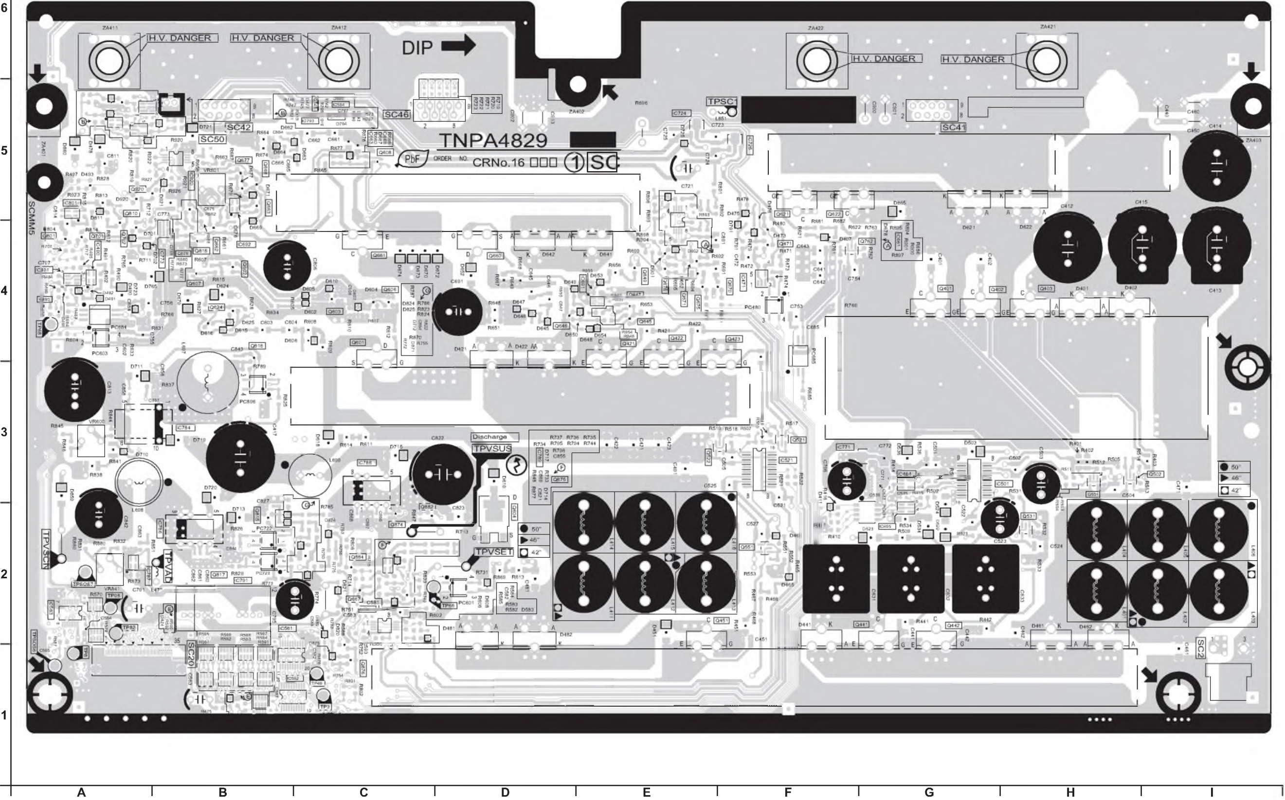
SC-BOARD (COMPONENT SIDE) TXNSC11XBH
