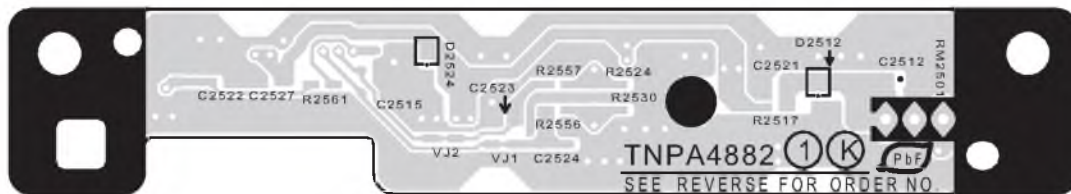
K-BOARD (FOIL SIDE) TXN/K1ETUR
