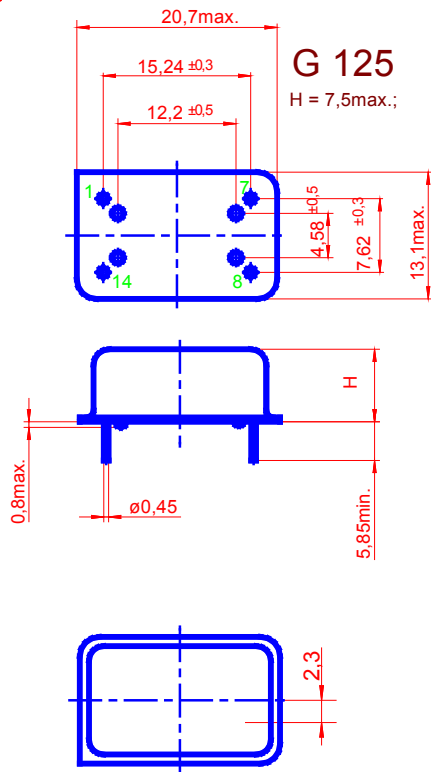
Type A Code Height "H" Pin Length "L" 0 7.5 5.85 1 8.0 5.85 2 10.1 5.85
