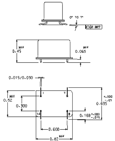
Type C Code Height "H" Pin Length "L" 4 0.45 NA
