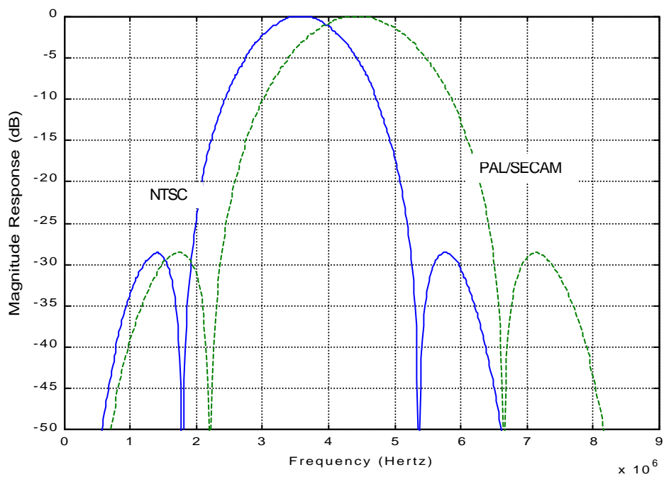
Chroma Band Pass Filter Curves
