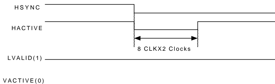
Figure 9b. VBI HACTIVE timing during VBI lines
