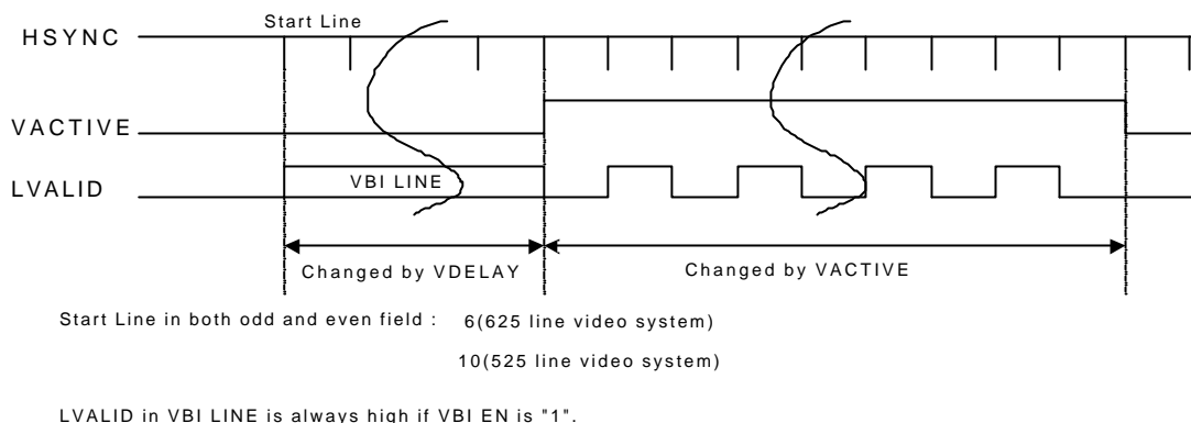
Figure 10. VACTIVE and LVALID timing
