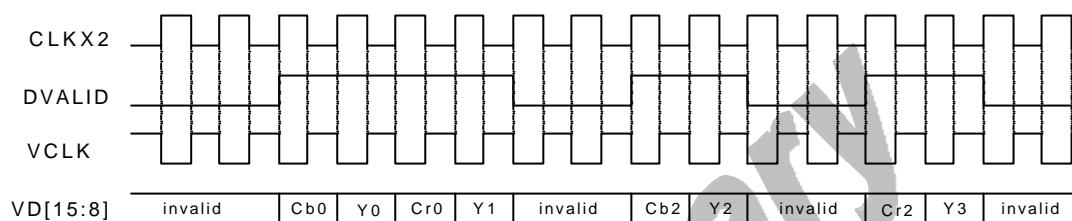
Figure 11b. 8-bit DVALID second format timing
