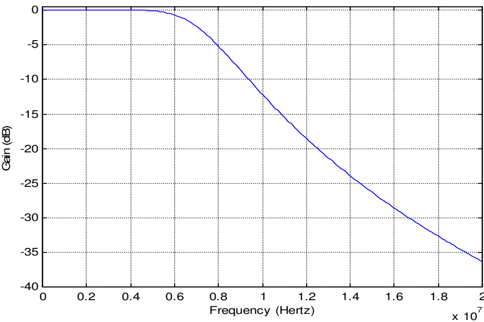
Decimation filter
