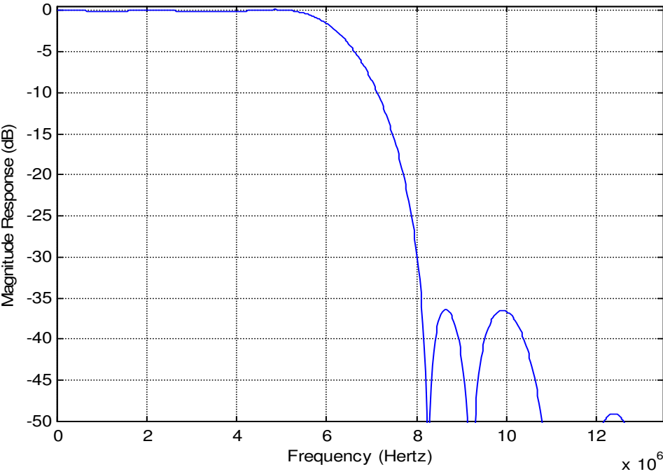
Decimation filter
