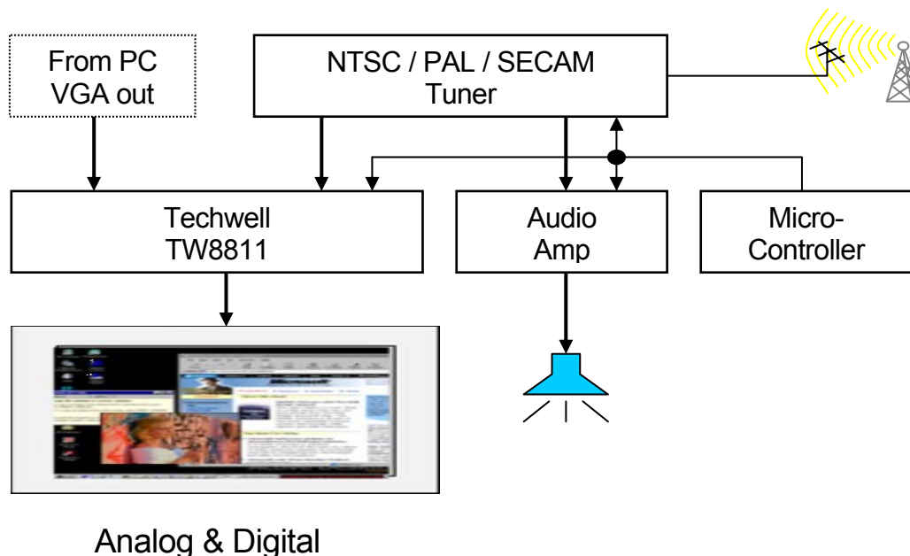
TW8811 Flat Panel TV or TV + PC Monitor system
