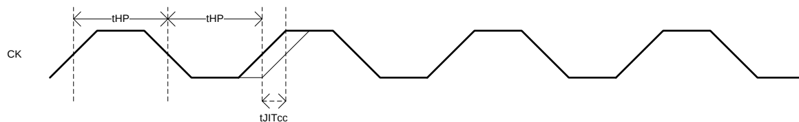
FIGURE 38. DDR2 INTERFACE CLOCK TIMING
