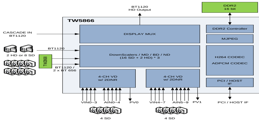
FIGURE 1. TW5866 BLOCK DIAGRAM
