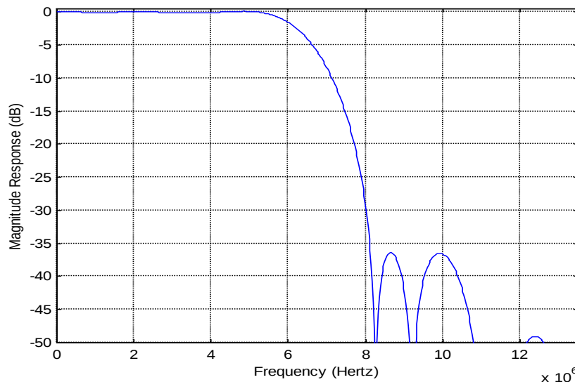
FIGURE 6. THE CHARACTERISTIC OF DECIMATION FILTER
