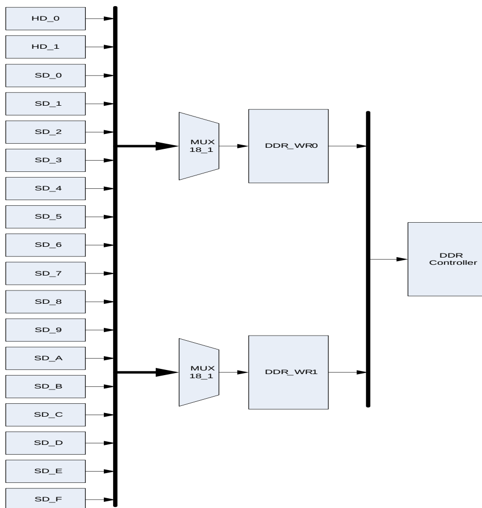
FIGURE 30. MJPEG ENCODING CAPTURE PATH CHANNEL SELECTION
