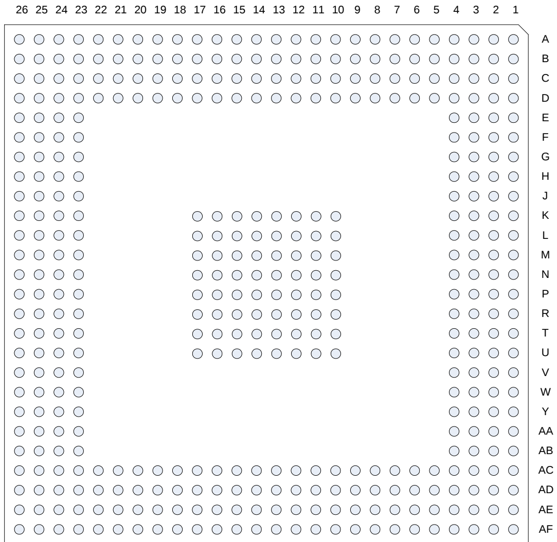
FIGURE 4. TW5866 BALL ARRANGEMENT (BOTTOM VIEW)
