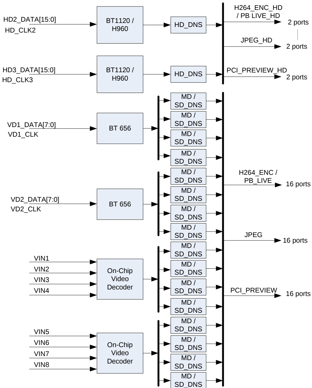
FIGURE 25. THE PRE-PROCESSING MODULE
