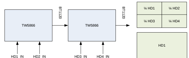
FIGURE 24. TWO TW5866 CASCADE TO SUPPORT SINGLE HD WINDOWS OR 4 WINDOWS IN 1/4 HD
