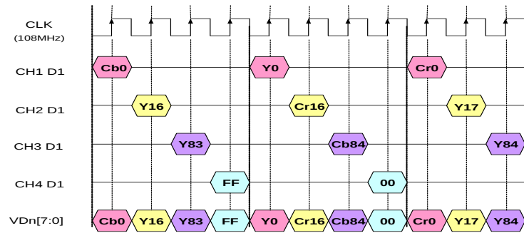
FIGURE 13. PIN OUTPUT TIMING OF 108MHZ 4 CH D1 TIME-DIVISION-MULTIPLEXED VIDEO DATA WITH 108MHZ CLOCK
