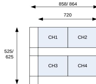
FIGURE 19. HALF D1 FIELD INTERLEAVED: TYPE 6
