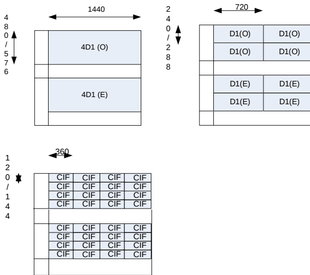
FIGURE 20. 4D1 OUTPUT FORMAT: SINGLE CHANNEL (LEFT), QUAD CHANNEL (RIGHT), AND 16 CHANNEL (BOTTOM)
