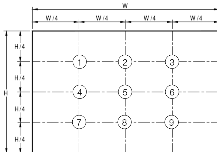
Figure 3. Uniformity Measurement Locations (9 points)
