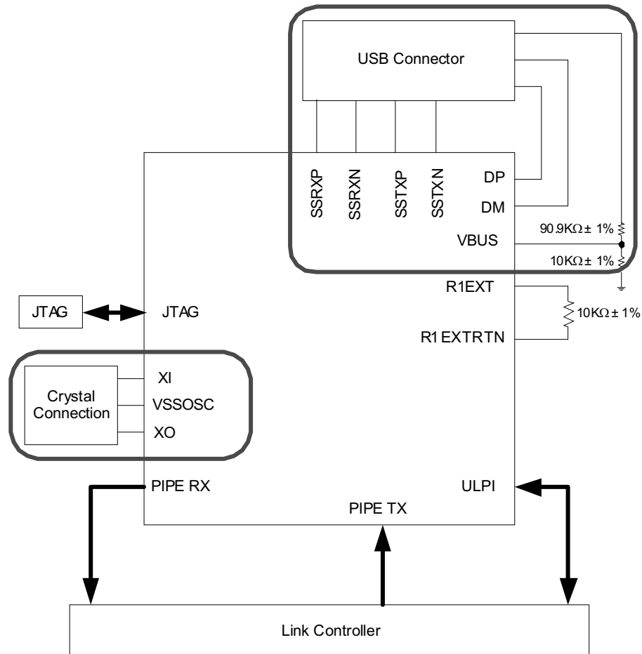
Figure 6-2. Analog Pin Connections
