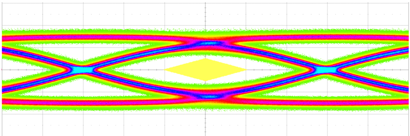
Figure 6-6. Super Speed Eye Diagram
