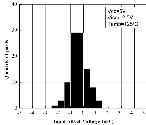
Figure 3. Input offset voltage distribution at T = 125^\circ\text{C}
