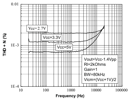
Figure 14. Distortion + noise vs. frequency
