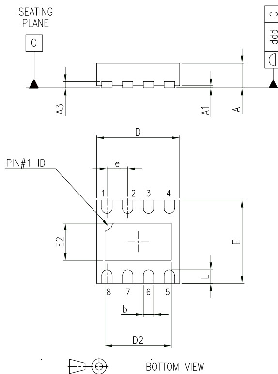
Figure 21. DFN8 2 x 2 package outline
