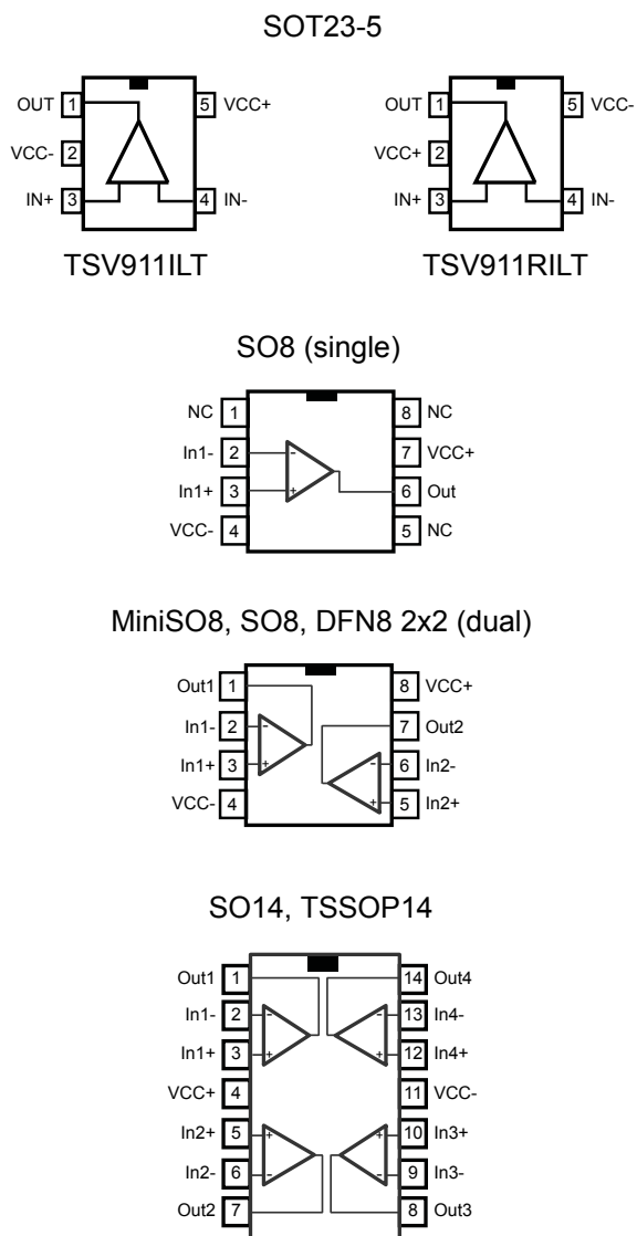
Figure 1. Pin connections for each package (top view)
