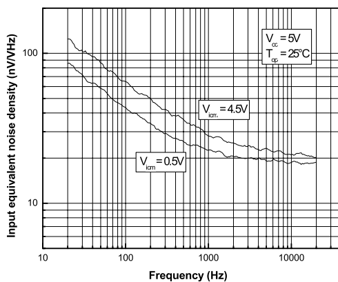
Figure 16. Noise vs. frequency
