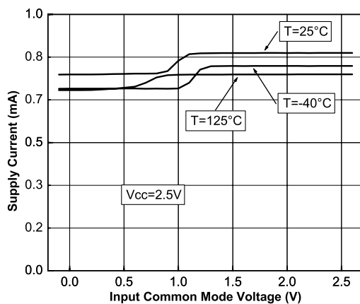
Figure 4. Supply current vs. input common-mode voltage at V_{CC} = 2.5\text{ V}
