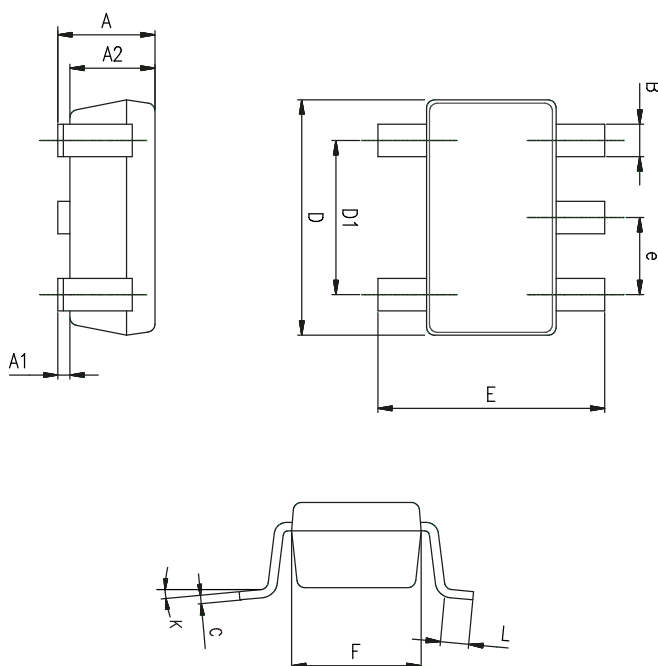
Figure 20. SOT23-5 package outline
