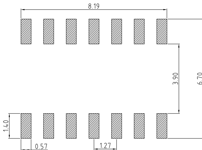
Figure 28. SO-14 recommended footprint
