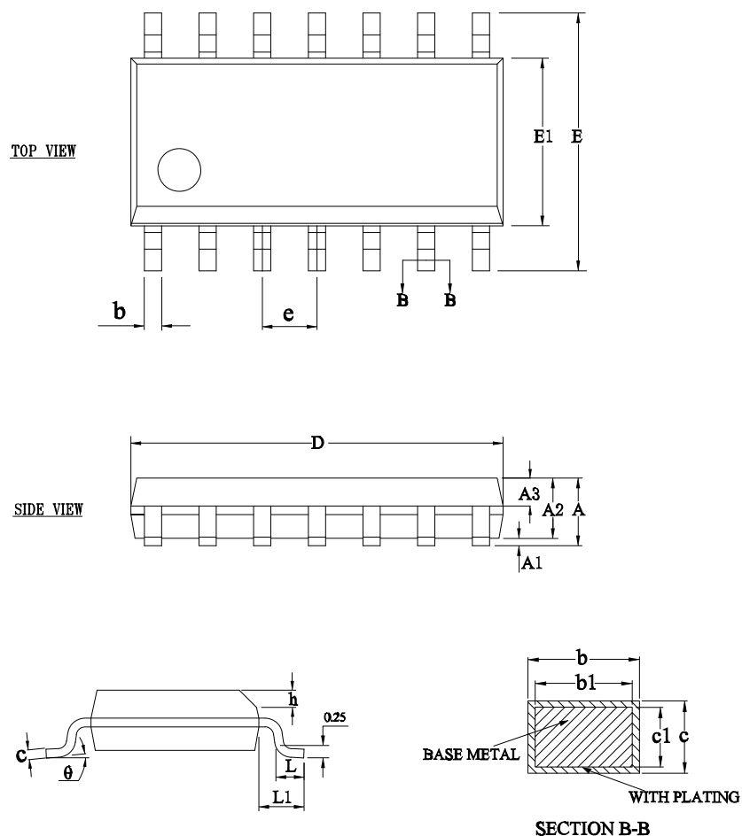
Figure 27. SO-14 package outline
