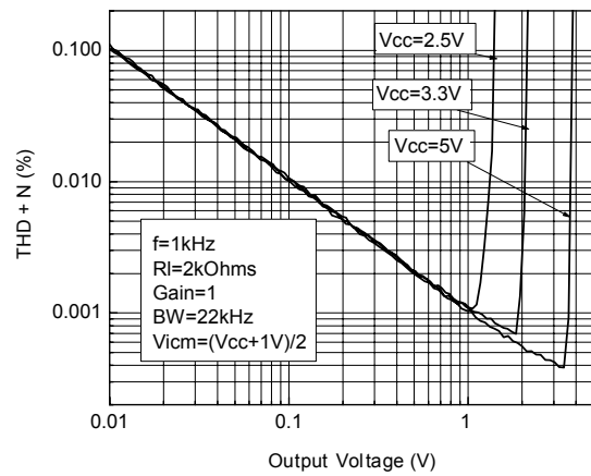
Figure 15. Distortion + noise vs. output voltage
