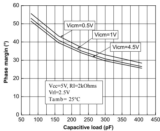
Figure 10. Phase margin vs. capacitive load
