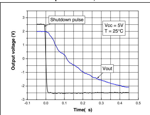
Figure 21. Turn-off time, V_{\text{CC}} = 5 V, V_{\text{out}} pulled down, T = 25^\circ\text{C}
