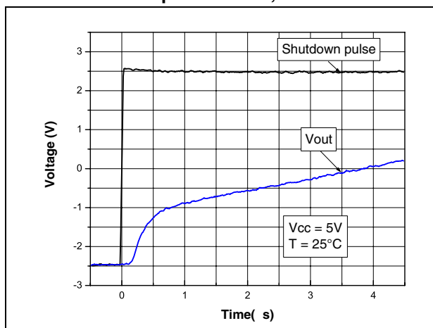
Figure 20. Turn-on time, V_{\text{CC}} = 5 V, V_{\text{out}} pulled down, T = 25^\circ\text{C}
