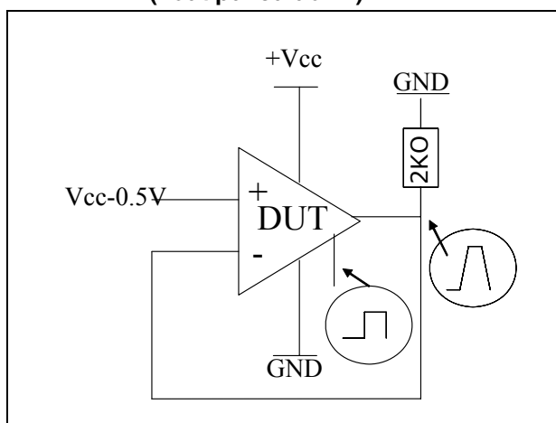
Figure 18. Test configuration for turn-on time ( V_{\text{out}} pulled down)
