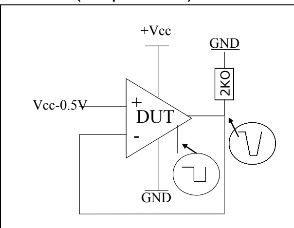
Figure 19. Test configuration for turn-off time ( V_{\text{out}} pulled down)
