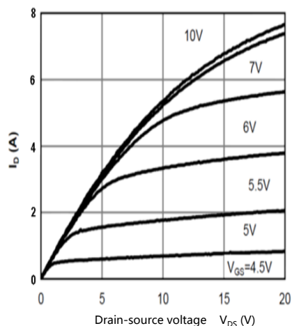
Figure 2: On-Region Characteristics@125°C
