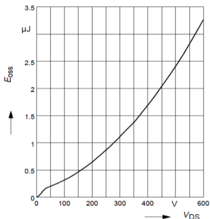
Figure 9: C_{oss} stored Energy
