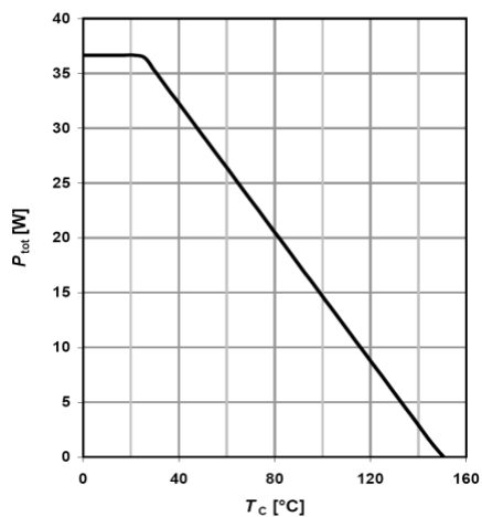
Figure 3: Power Dissipation
