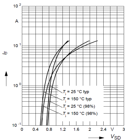
Figure 6: Body-Diode Characteristics
