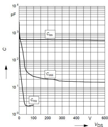
Figure 8: Capacitance Characteristics
