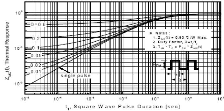
Figure 11-1. Transient Thermal Response Curve for TSP640M
