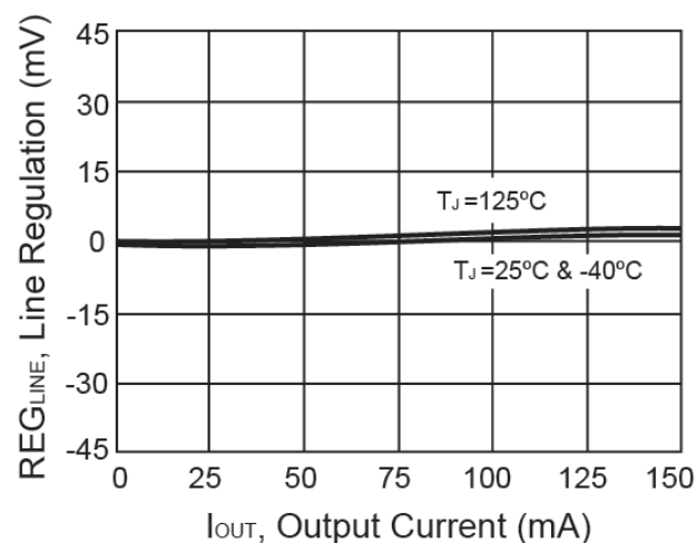
Figure 6. Line Regulation vs. Output Current
