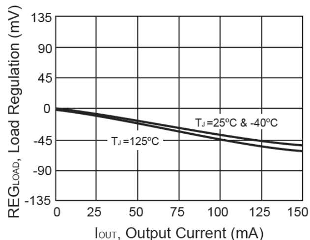
Figure 5. Load Regulation vs. Output Current
