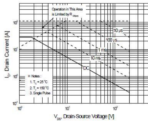
Figure 9-2. Maximum Safe Operating Area for TSF32N20M
