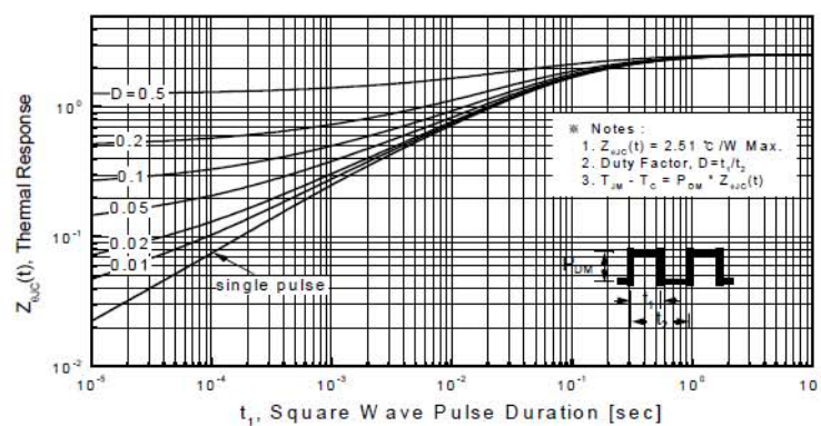
Figure 11-2. Transient Thermal Response Curve for TSF32N20M
