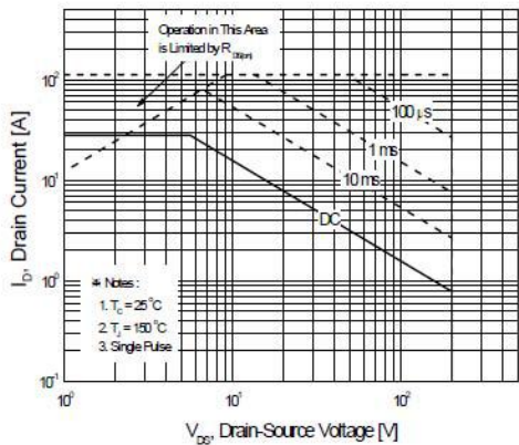
Figure 9-1. Maximum Safe Operating Area for TSP32N20M
