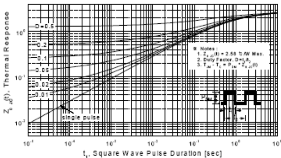
Figure 11-2. Transient Thermal Response Curve for TSF13N50M
