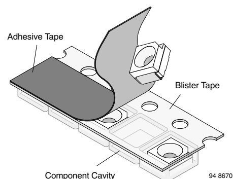
Figure 9. Blister Tape
