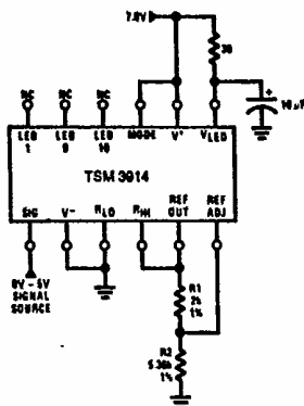
Linear Bar Graph (5V Full-Scale)
