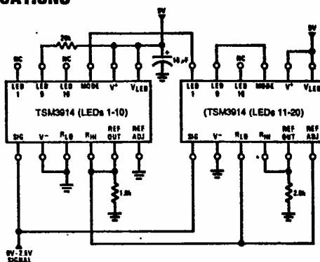
20-Segment Linear Dot Graph (2.5V Full-Scale)
