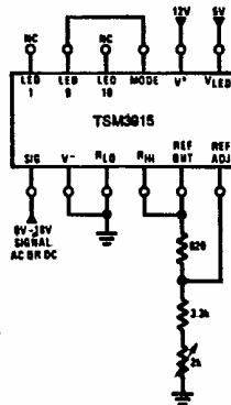
Logarithmic Audio Dot Graph (10V Full-Scale)
