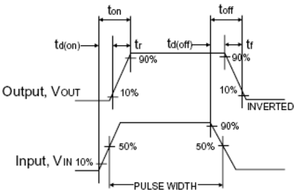
Switchin Waveforms
