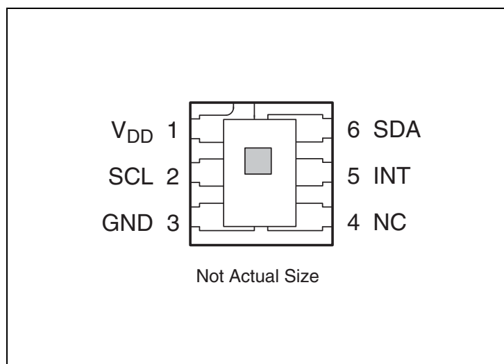
Figure 3: Package FN Dual Flat No-Lead (Top View)
