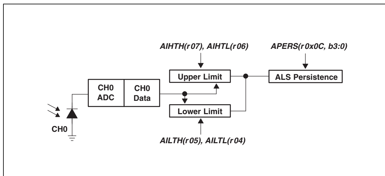
Figure 17: Programmable Interrupt
