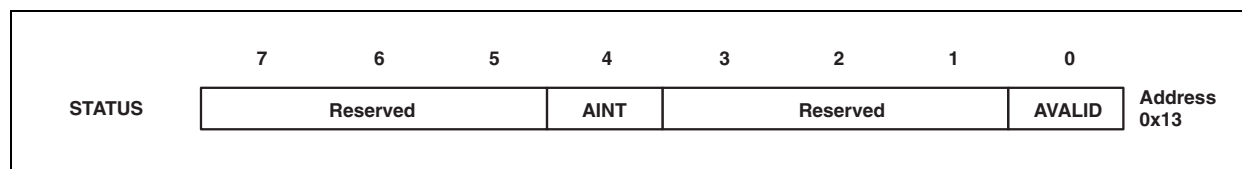
Figure 30: Status Register
