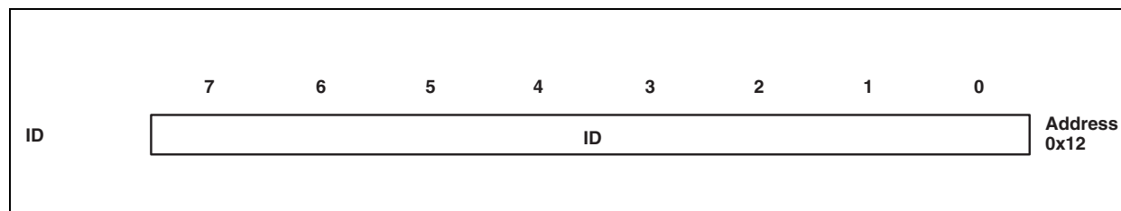
Figure 29: ID Register
