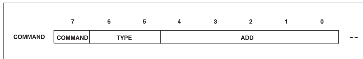
Figure 21: Command Register
