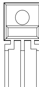
PACKAGE SM SURFACE MOUNT SIDELOOKER (FRONT VIEW)
